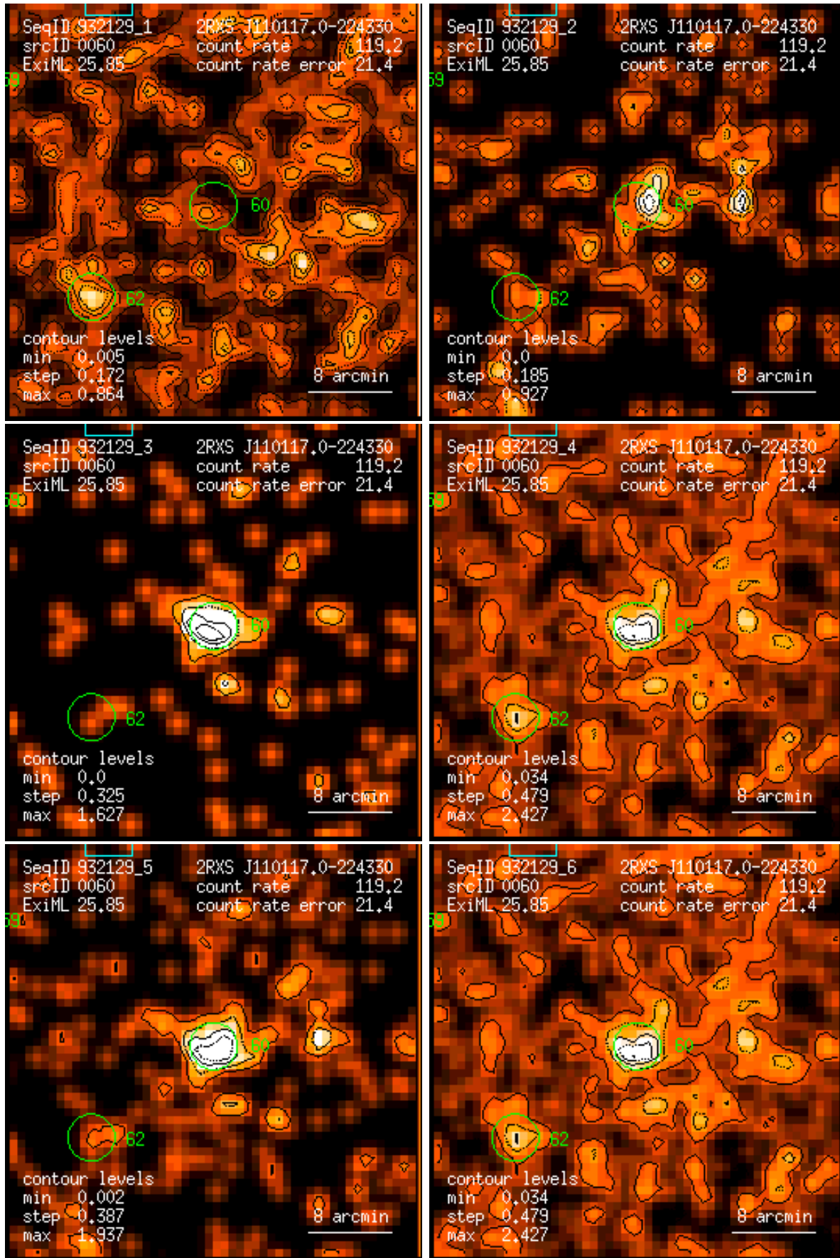
Figure 60: RASS 932129: detection 0060: band rate images, Gaussian filter: (1) PSPC channels 11 – 41, (2) 52 – 90, (3) 91 – 201, (4) 11 – 235, (5) 52 – 201, (6) 11 – 201. Broad band rates in counts/ks. Band rate contour levels in counts/ks/arcmin 2 .
