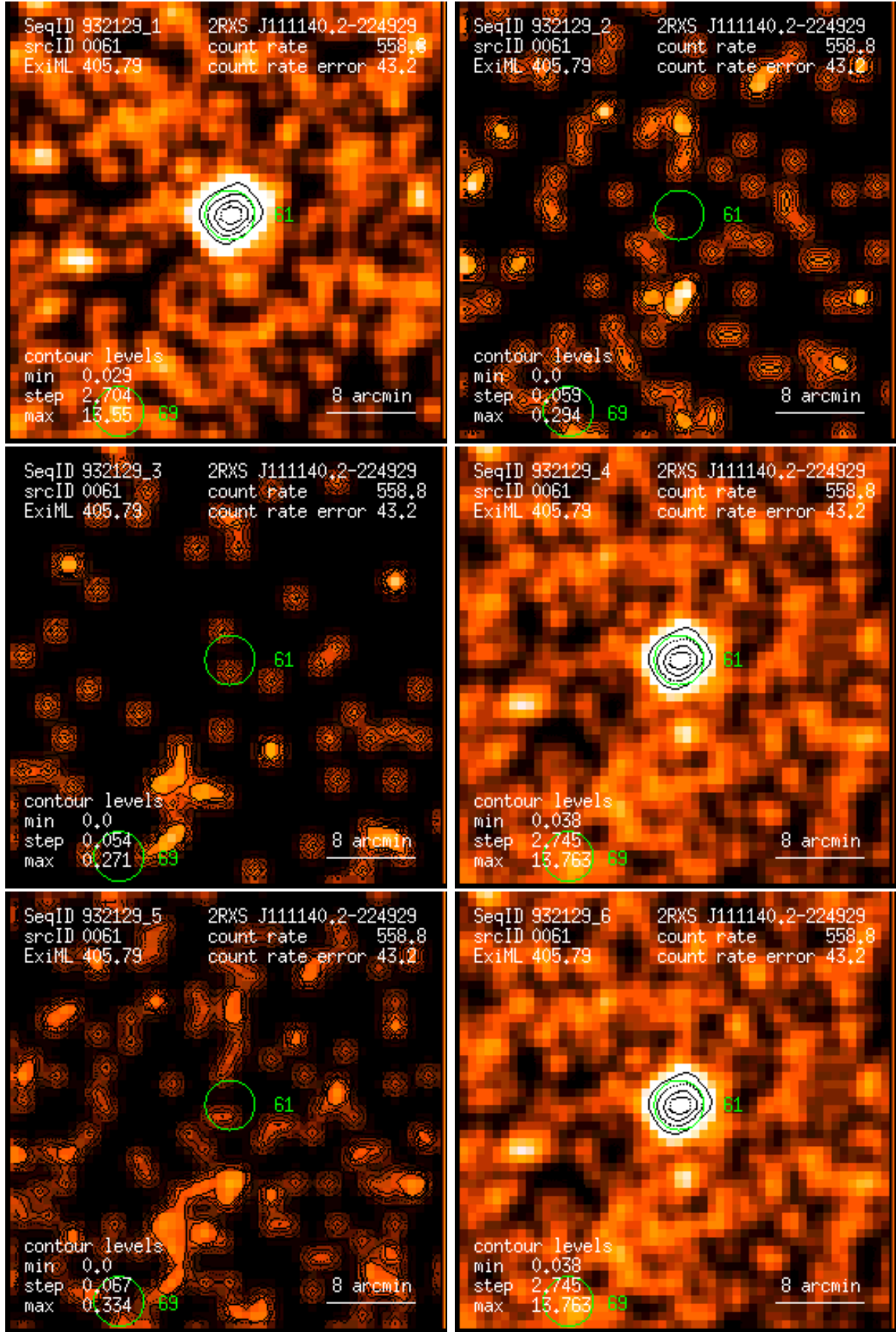
Figure 61: RASS 932129: detection 0061: band rate images, Gaussian filter: (1) PSPC channels 11 – 41, (2) 52 – 90, (3) 91 – 201, (4) 11 – 235, (5) 52 – 201, (6) 11 – 201. Broad band rates in counts/ks. Band rate contour levels in counts/ks/arcmin 2 .
