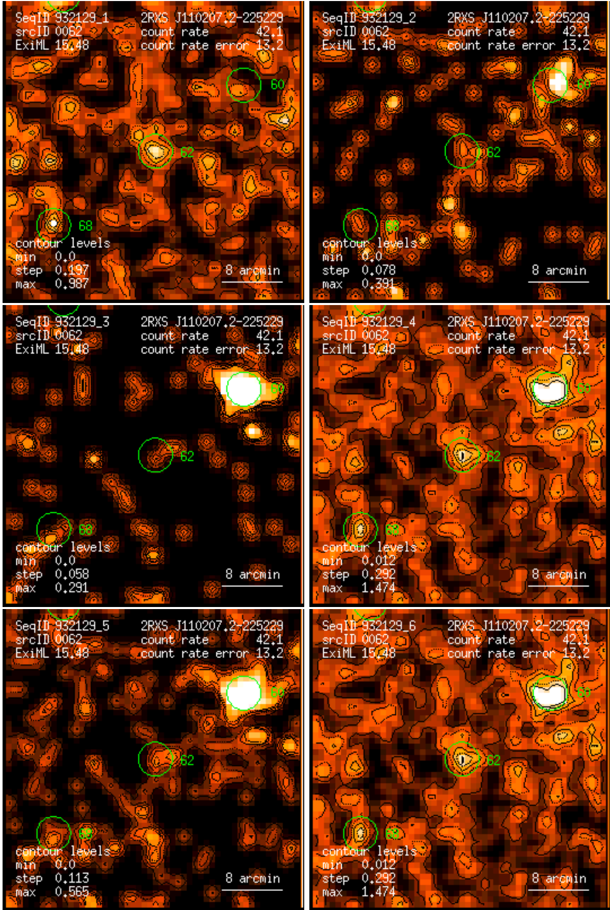
Figure 62: RASS 932129: detection 0062: band rate images, Gaussian filter: (1) PSPC channels 11 – 41, (2) 52 – 90, (3) 91 – 201, (4) 11 – 235, (5) 52 – 201, (6) 11 – 201. Broad band rates in counts/ks. Band rate contour levels in counts/ks/arcmin 2 .
