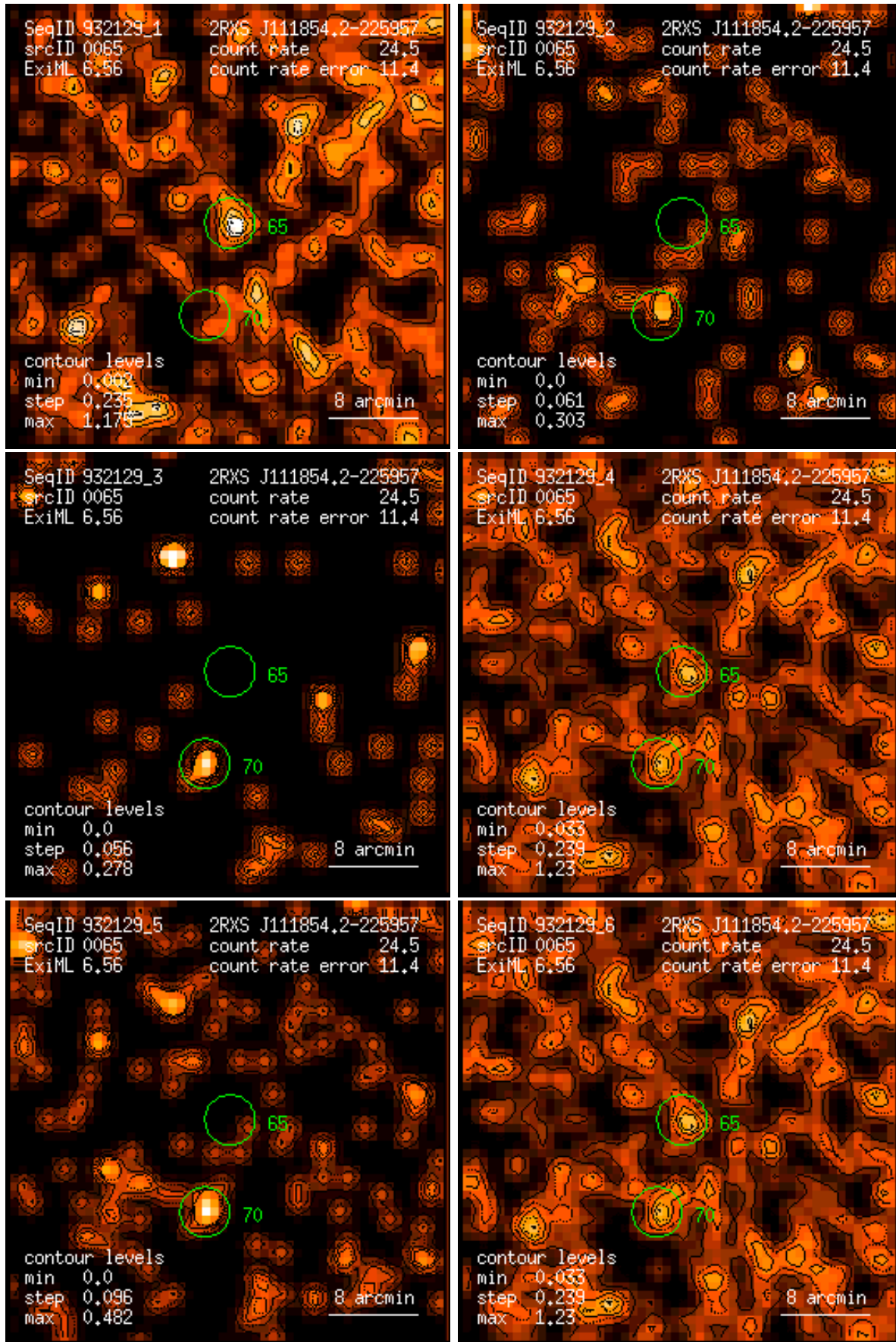
Figure 65: RASS 932129: detection 0065: band rate images, Gaussian filter: (1) PSPC channels 11 – 41, (2) 52 – 90, (3) 91 – 201, (4) 11 – 235, (5) 52 – 201, (6) 11 – 201. Broad band rates in counts/ks. Band rate contour levels in counts/ks/arcmin 2 .
