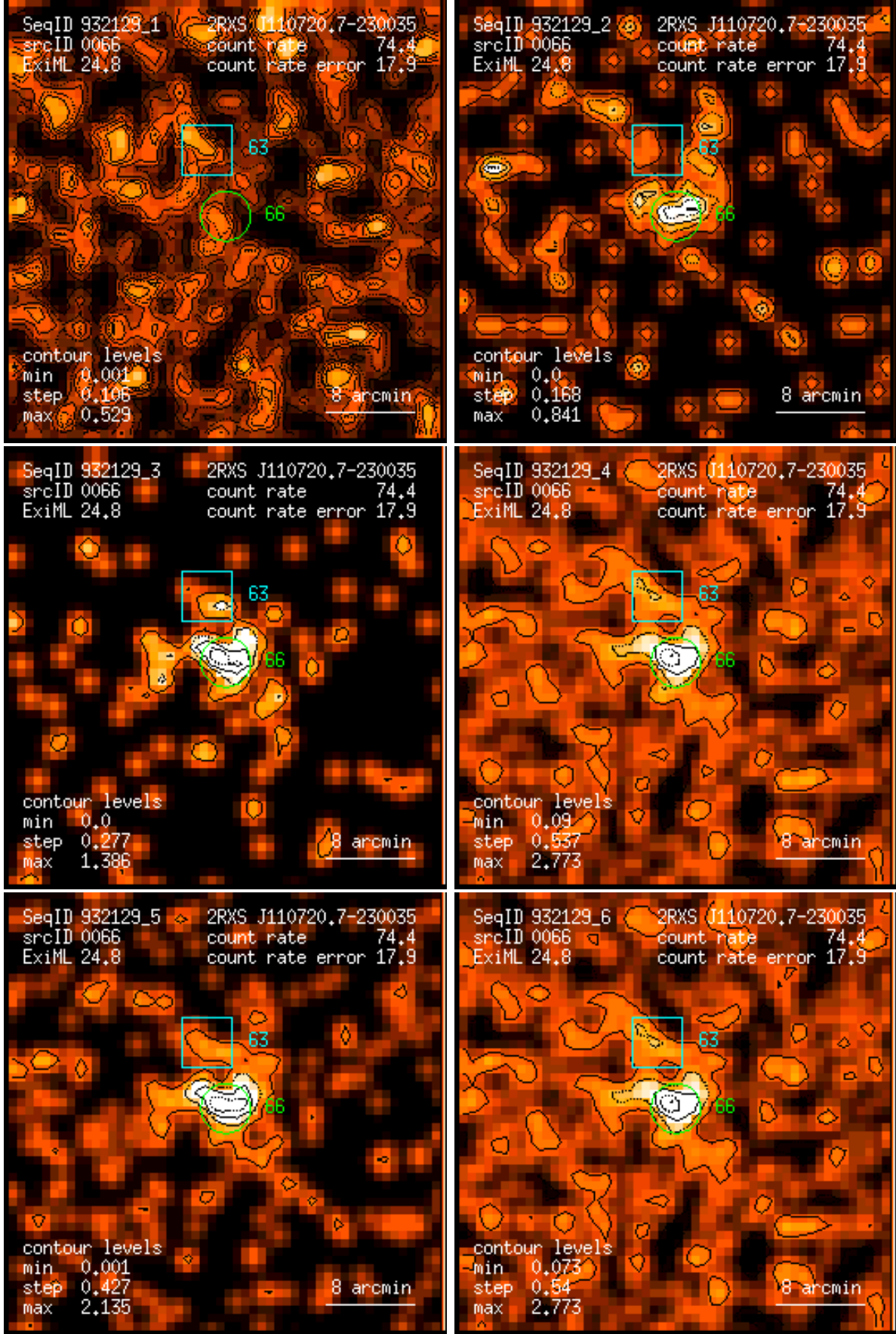
Figure 66: RASS 932129: detection 0066: band rate images, Gaussian filter: (1) PSPC channels 11 – 41, (2) 52 – 90, (3) 91 – 201, (4) 11 – 235, (5) 52 – 201, (6) 11 – 201. Broad band rates in counts/ks. Band rate contour levels in counts/ks/arcmin 2 .
