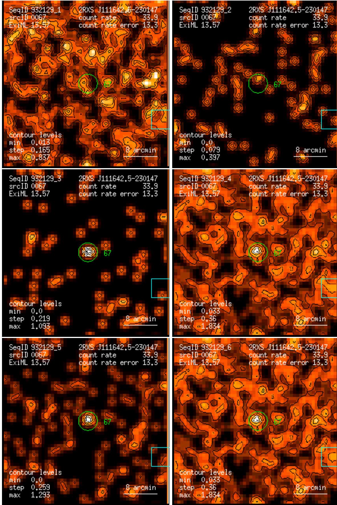
Figure 67: RASS 932129: detection 0067: band rate images, Gaussian filter: (1) PSPC channels 11 – 41, (2) 52 – 90, (3) 91 – 201, (4) 11 – 235, (5) 52 – 201, (6) 11 – 201. Broad band rates in counts/ks. Band rate contour levels in counts/ks/arcmin 2 .
