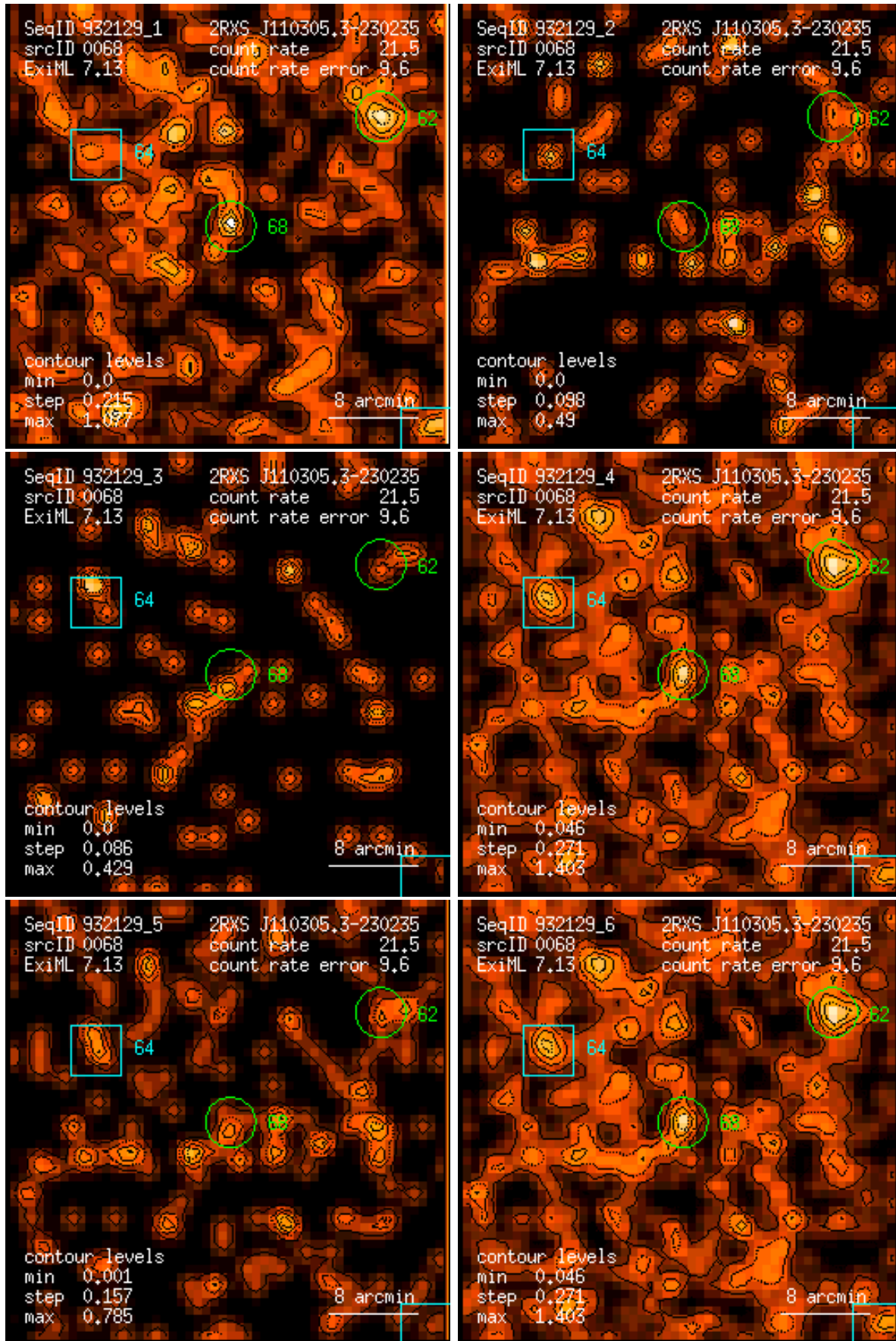
Figure 68: RASS 932129: detection 0068: band rate images, Gaussian filter: (1) PSPC channels 11 – 41, (2) 52 – 90, (3) 91 – 201, (4) 11 – 235, (5) 52 – 201, (6) 11 – 201. Broad band rates in counts/ks. Band rate contour levels in counts/ks/arcmin 2 .
