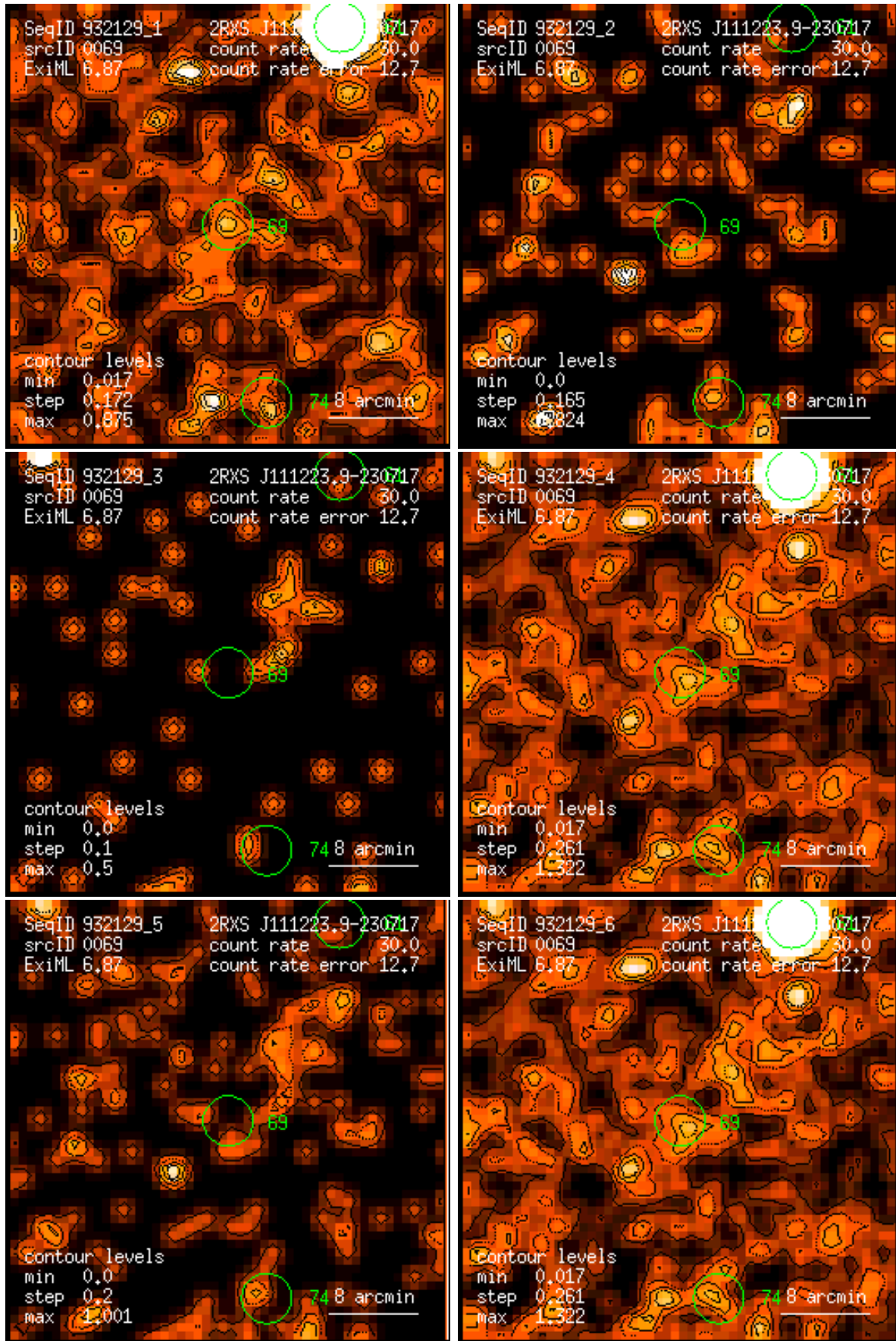
Figure 69: RASS 932129: detection 0069: band rate images, Gaussian filter: (1) PSPC channels 11 – 41, (2) 52 – 90, (3) 91 – 201, (4) 11 – 235, (5) 52 – 201, (6) 11 – 201. Broad band rates in counts/ks. Band rate contour levels in counts/ks/arcmin 2 .
