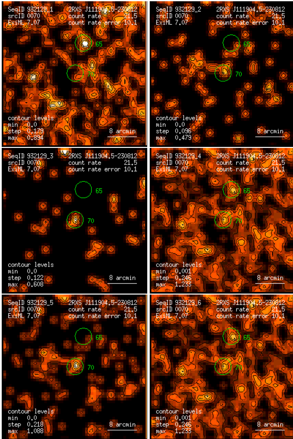
Figure 70: RASS 932129: detection 0070: band rate images, Gaussian filter: (1) PSPC channels 11 – 41, (2) 52 – 90, (3) 91 – 201, (4) 11 – 235, (5) 52 – 201, (6) 11 – 201. Broad band rates in counts/ks. Band rate contour levels in counts/ks/arcmin 2 .
