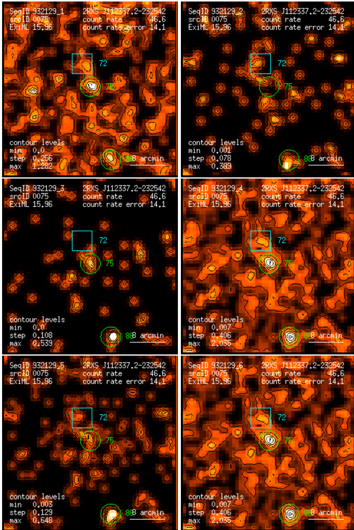
Figure 75: RASS 932129: detection 0075: band rate images, Gaussian filter: (1) PSPC channels 11 – 41, (2) 52 – 90, (3) 91 – 201, (4) 11 – 235, (5) 52 – 201, (6) 11 – 201. Broad band rates in counts/ks. Band rate contour levels in counts/ks/arcmin 2 .
