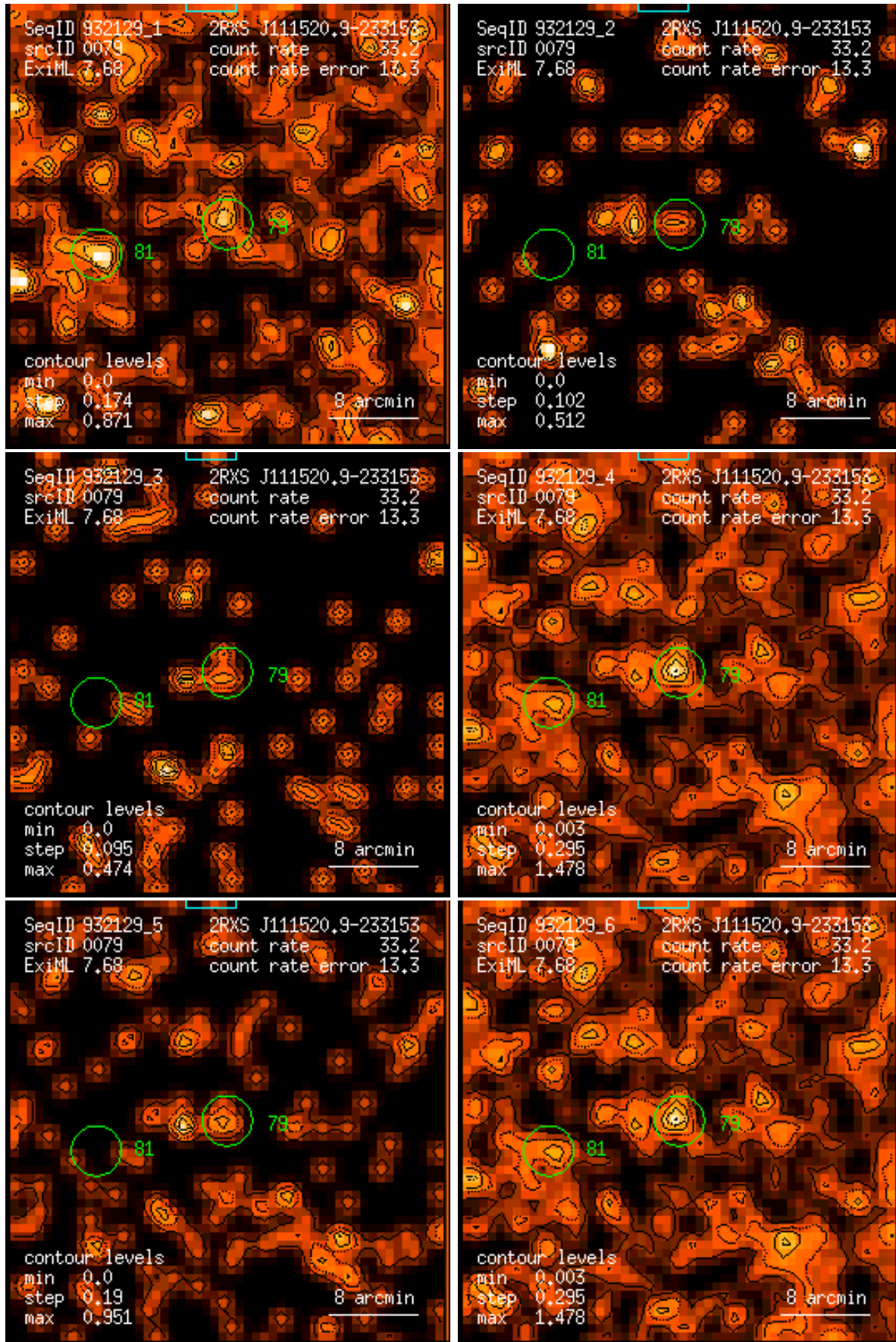
Figure 79: RASS 932129: detection 0079: band rate images, Gaussian filter: (1) PSPC channels 11 – 41, (2) 52 – 90, (3) 91 – 201, (4) 11 – 235, (5) 52 – 201, (6) 11 – 201. Broad band rates in counts/ks. Band rate contour levels in counts/ks/arcmin 2 .
