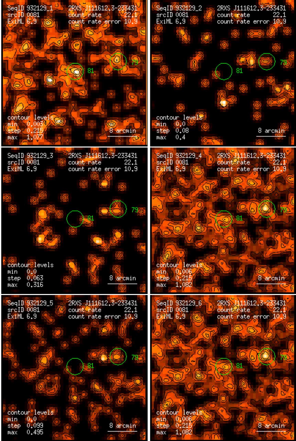
Figure 81: RASS 932129: detection 0081: band rate images, Gaussian filter: (1) PSPC channels 11 – 41, (2) 52 – 90, (3) 91 – 201, (4) 11 – 235, (5) 52 – 201, (6) 11 – 201. Broad band rates in counts/ks. Band rate contour levels in counts/ks/arcmin 2 .
