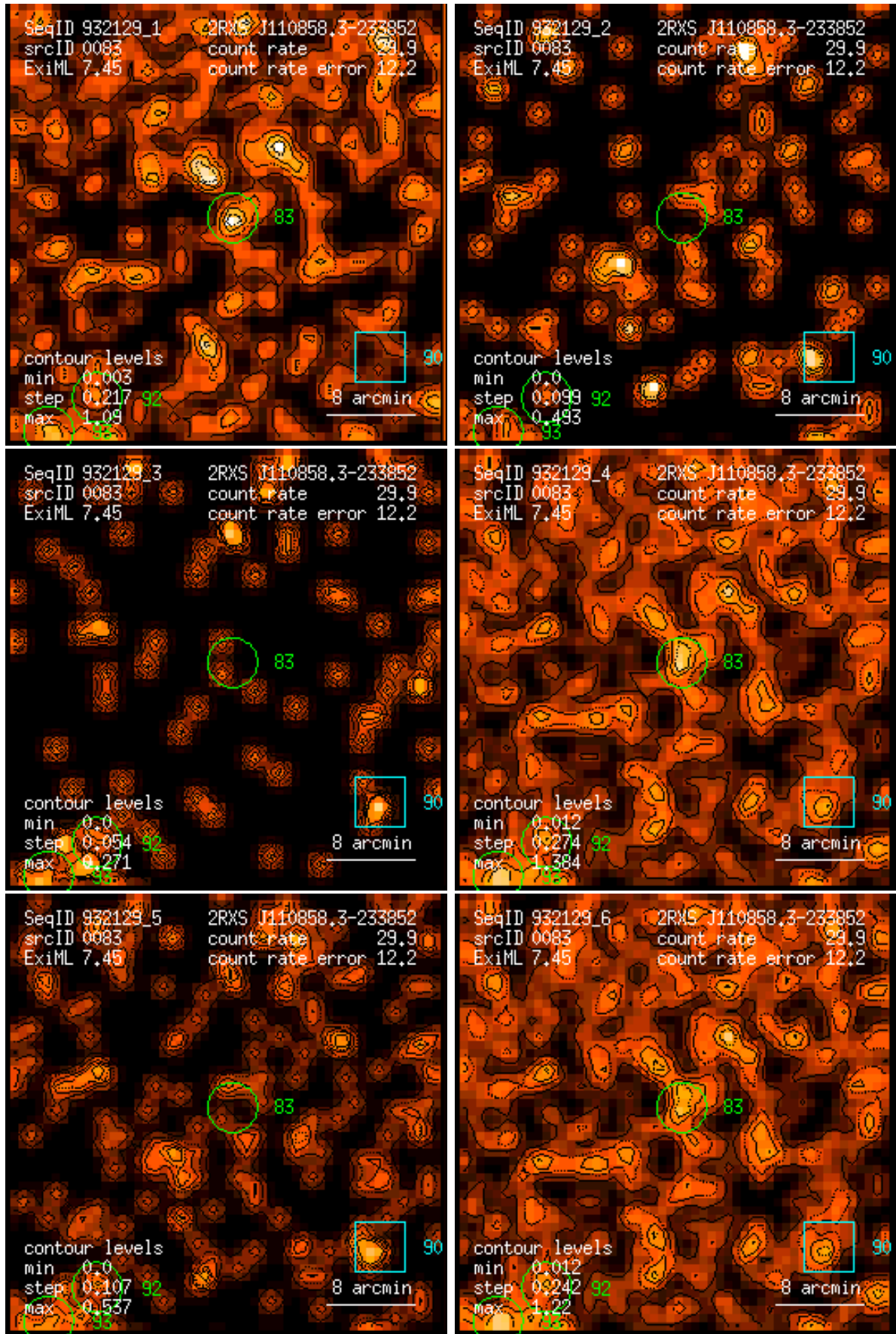
Figure 83: RASS 932129: detection 0083: band rate images, Gaussian filter: (1) PSPC channels 11 – 41, (2) 52 – 90, (3) 91 – 201, (4) 11 – 235, (5) 52 – 201, (6) 11 – 201. Broad band rates in counts/ks. Band rate contour levels in counts/ks/arcmin 2 .
