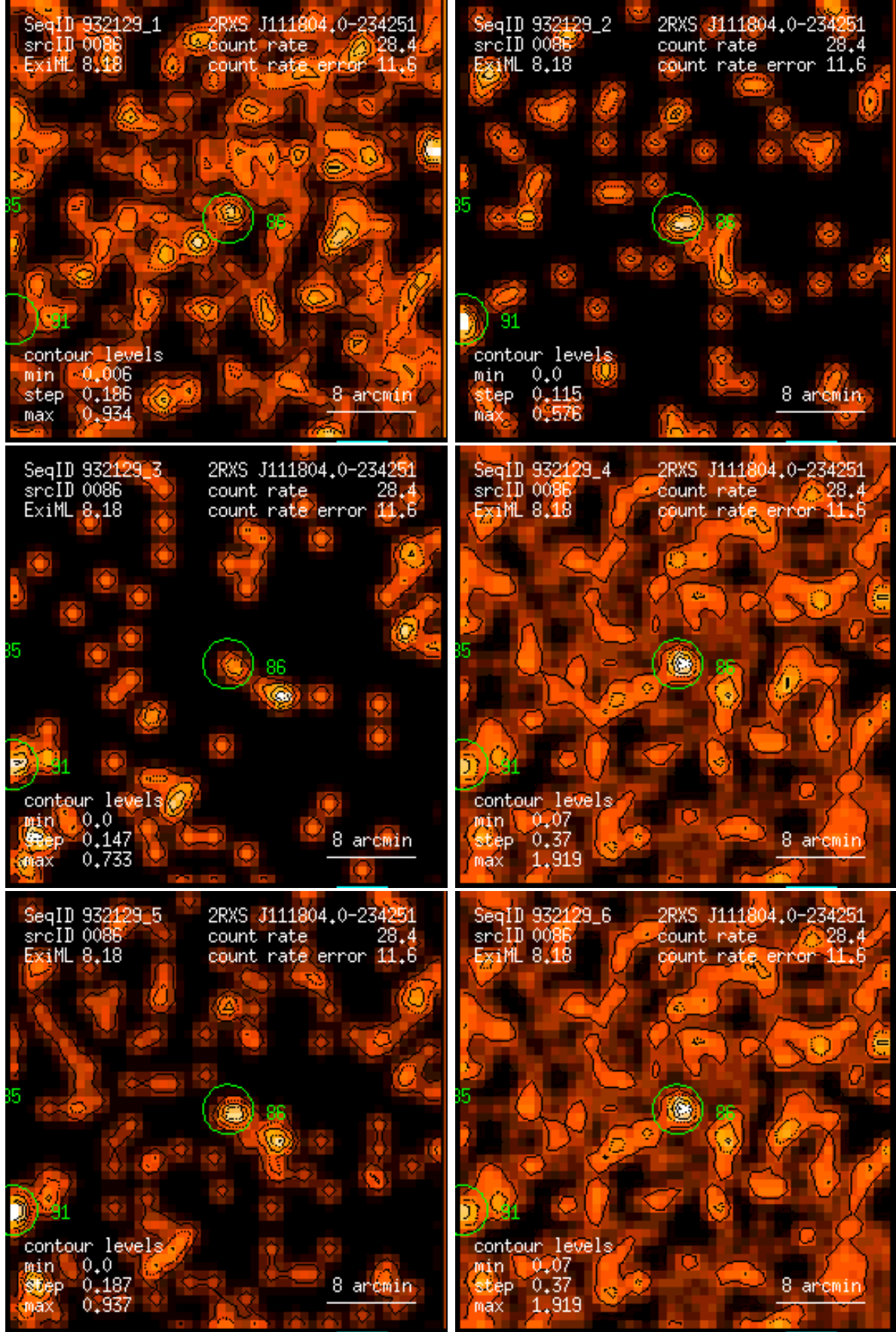
Figure 86: RASS 932129: detection 0086: band rate images, Gaussian filter: (1) PSPC channels 11 – 41, (2) 52 – 90, (3) 91 – 201, (4) 11 – 235, (5) 52 – 201, (6) 11 – 201. Broad band rates in counts/ks. Band rate contour levels in counts/ks/arcmin 2 .
