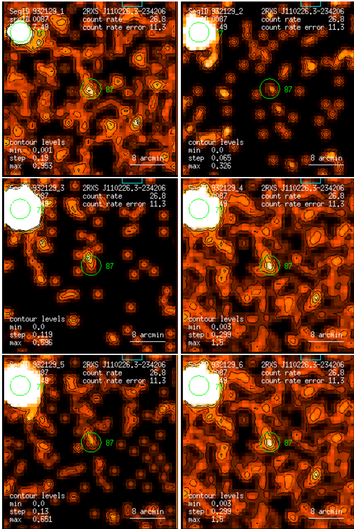
Figure 87: RASS 932129: detection 0087: band rate images, Gaussian filter: (1) PSPC channels 11 – 41, (2) 52 – 90, (3) 91 – 201, (4) 11 – 235, (5) 52 – 201, (6) 11 – 201. Broad band rates in counts/ks. Band rate contour levels in counts/ks/arcmin 2 .
