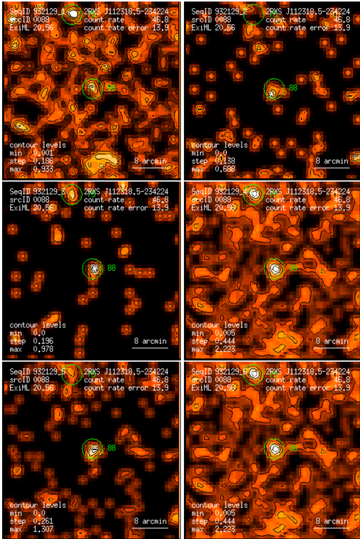
Figure 88: RASS 932129: detection 0088: band rate images, Gaussian filter: (1) PSPC channels 11 – 41, (2) 52 – 90, (3) 91 – 201, (4) 11 – 235, (5) 52 – 201, (6) 11 – 201. Broad band rates in counts/ks. Band rate contour levels in counts/ks/arcmin 2 .
