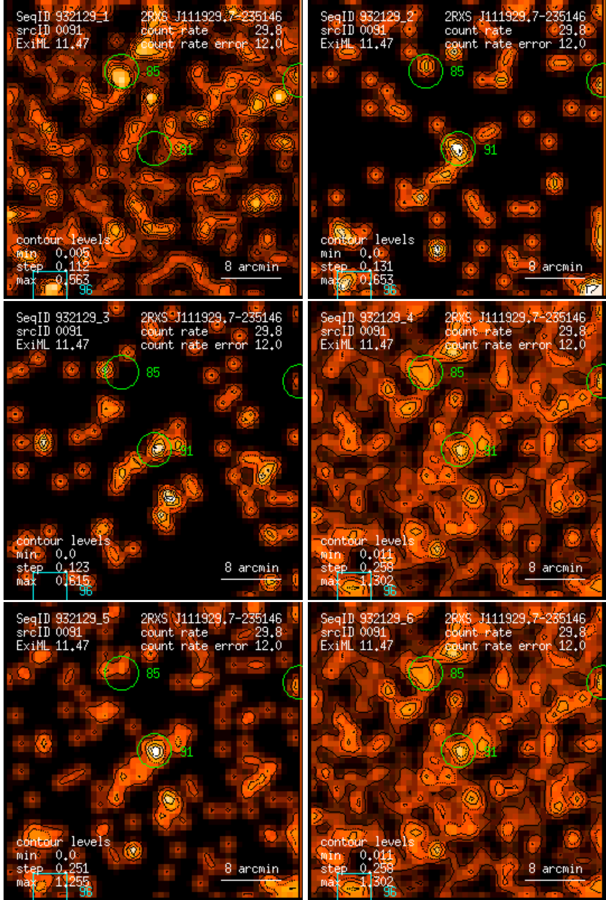
Figure 91: RASS 932129: detection 0091: band rate images, Gaussian filter: (1) PSPC channels 11 – 41, (2) 52 – 90, (3) 91 – 201, (4) 11 – 235, (5) 52 – 201, (6) 11 – 201. Broad band rates in counts/ks. Band rate contour levels in counts/ks/arcmin 2 .
