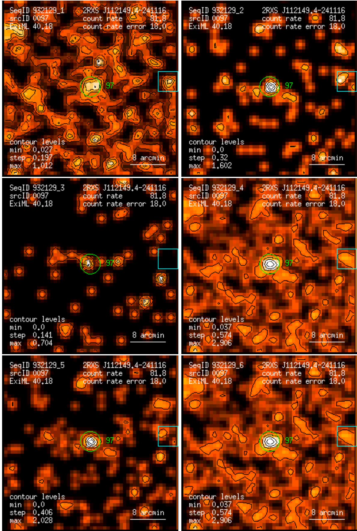
Figure 97: RASS 932129: detection 0097: band rate images, Gaussian filter: (1) PSPC channels 11 – 41, (2) 52 – 90, (3) 91 – 201, (4) 11 – 235, (5) 52 – 201, (6) 11 – 201. Broad band rates in counts/ks. Band rate contour levels in counts/ks/arcmin 2 .
