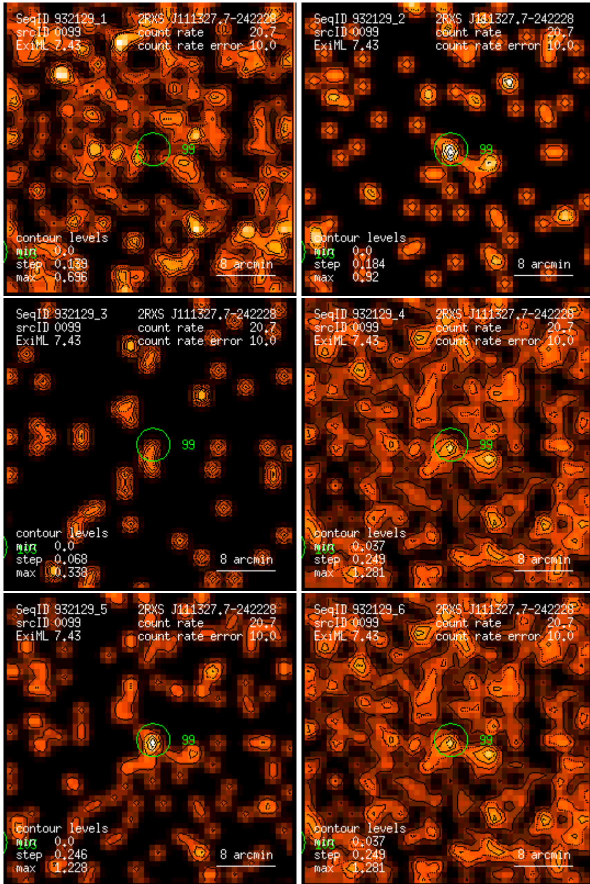
Figure 99: RASS 932129: detection 0099: band rate images, Gaussian filter: (1) PSPC channels 11 – 41, (2) 52 – 90, (3) 91 – 201, (4) 11 – 235, (5) 52 – 201, (6) 11 – 201. Broad band rates in counts/ks. Band rate contour levels in counts/ks/arcmin 2 .
