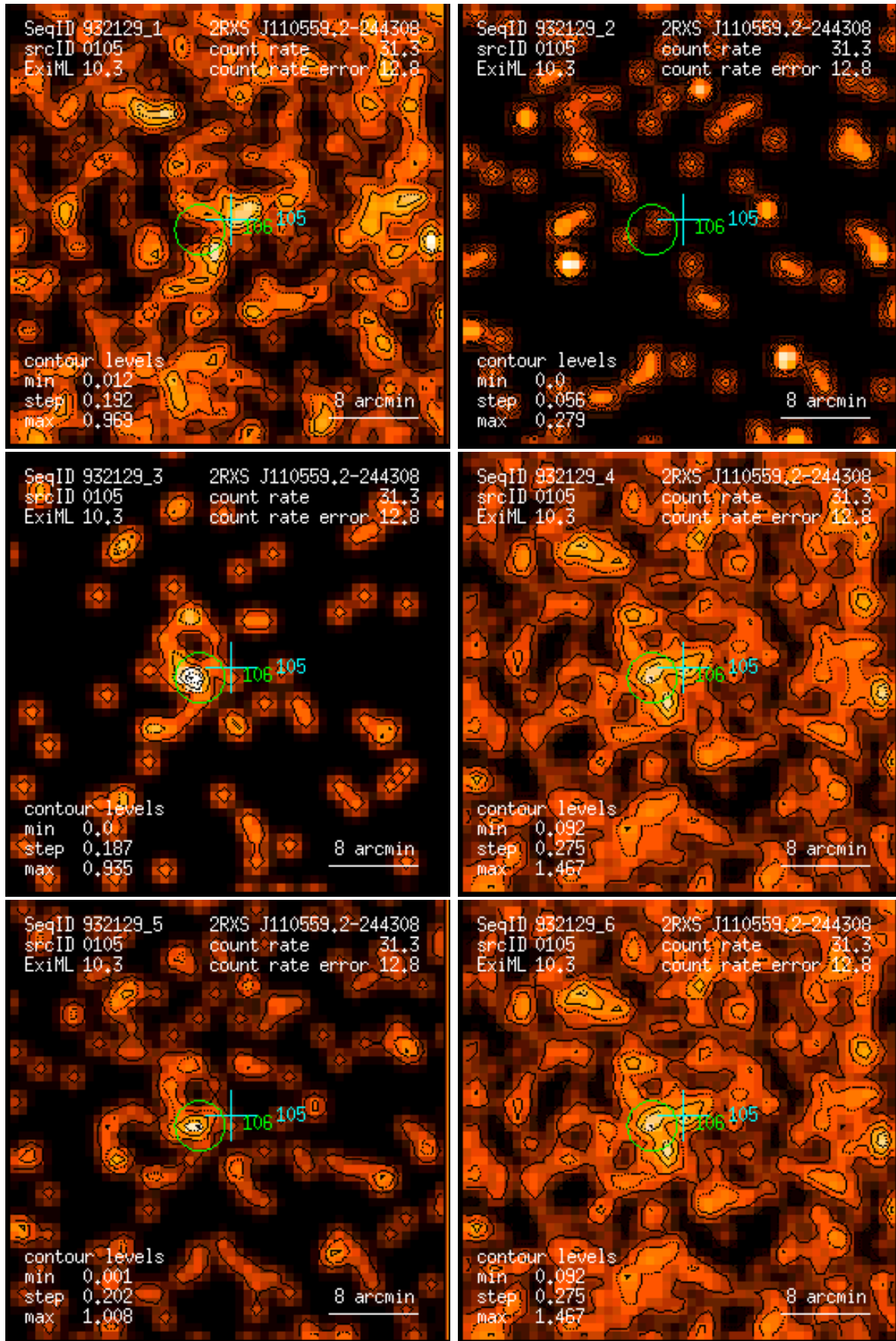
Figure 105: RASS 932129: detection 0105: band rate images, Gaussian filter: (1) PSPC channels 11 – 41, (2) 52 – 90, (3) 91 – 201, (4) 11 – 235, (5) 52 – 201, (6) 11 – 201. Broad band rates in counts/ks. Band rate contour levels in counts/ks/arcmin 2 .
