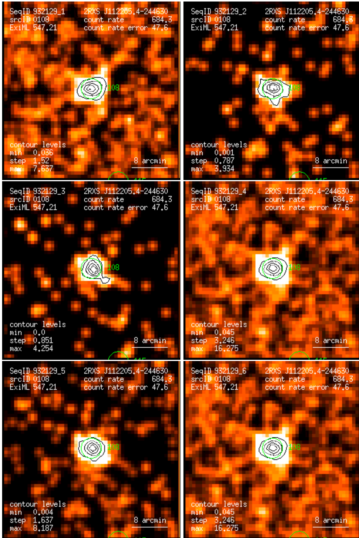
Figure 108: RASS 932129: detection 0108: band rate images, Gaussian filter: (1) PSPC channels 11 – 41, (2) 52 – 90, (3) 91 – 201, (4) 11 – 235, (5) 52 – 201, (6) 11 – 201. Broad band rates in counts/ks. Band rate contour levels in counts/ks/arcmin 2 .
