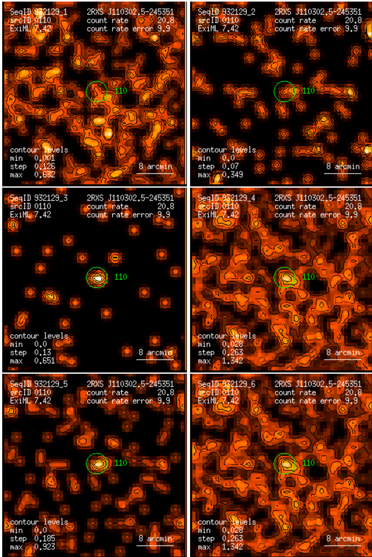
Figure 110: RASS 932129: detection 0110: band rate images, Gaussian filter: (1) PSPC channels 11 – 41, (2) 52 – 90, (3) 91 – 201, (4) 11 – 235, (5) 52 – 201, (6) 11 – 201. Broad band rates in counts/ks. Band rate contour levels in counts/ks/arcmin 2 .
