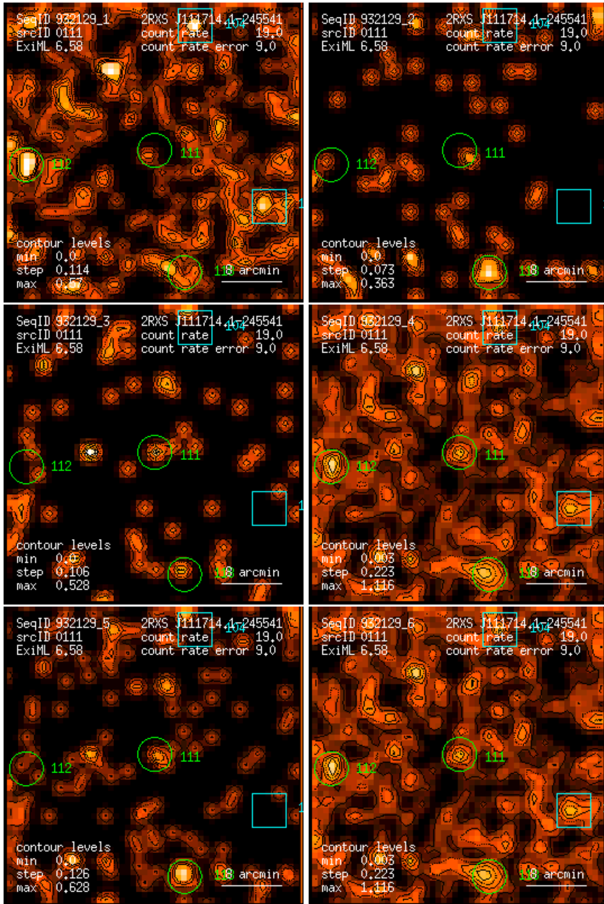
Figure 111: RASS 932129: detection 0111: band rate images, Gaussian filter: (1) PSPC channels 11 – 41, (2) 52 – 90, (3) 91 – 201, (4) 11 – 235, (5) 52 – 201, (6) 11 – 201. Broad band rates in counts/ks. Band rate contour levels in counts/ks/arcmin 2 .
