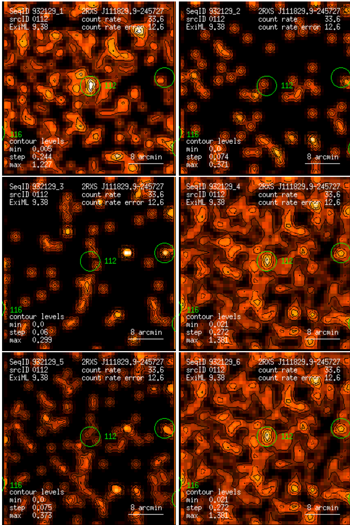
Figure 112: RASS 932129: detection 0112: band rate images, Gaussian filter: (1) PSPC channels 11 – 41, (2) 52 – 90, (3) 91 – 201, (4) 11 – 235, (5) 52 – 201, (6) 11 – 201. Broad band rates in counts/ks. Band rate contour levels in counts/ks/arcmin 2 .
