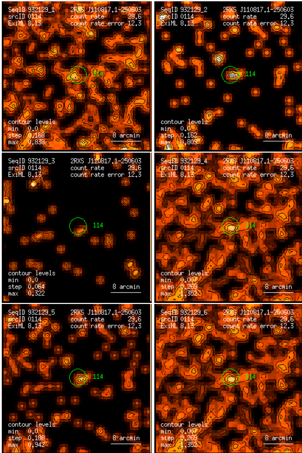
Figure 114: RASS 932129: detection 0114: band rate images, Gaussian filter: (1) PSPC channels 11 – 41, (2) 52 – 90, (3) 91 – 201, (4) 11 – 235, (5) 52 – 201, (6) 11 – 201. Broad band rates in counts/ks. Band rate contour levels in counts/ks/arcmin 2 .
