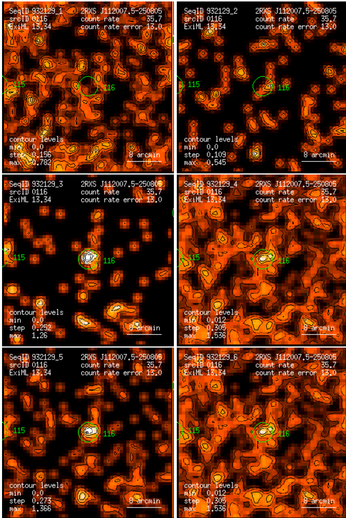
Figure 116: RASS 932129: detection 0116: band rate images, Gaussian filter: (1) PSPC channels 11 – 41, (2) 52 – 90, (3) 91 – 201, (4) 11 – 235, (5) 52 – 201, (6) 11 – 201. Broad band rates in counts/ks. Band rate contour levels in counts/ks/arcmin 2 .
