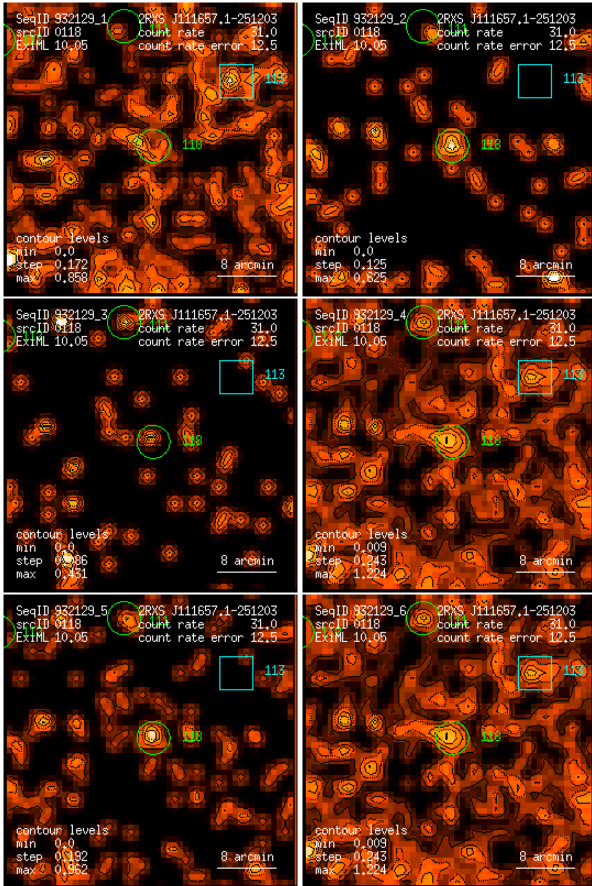
Figure 118: RASS 932129: detection 0118: band rate images, Gaussian filter: (1) PSPC channels 11 – 41, (2) 52 – 90, (3) 91 – 201, (4) 11 – 235, (5) 52 – 201, (6) 11 – 201. Broad band rates in counts/ks. Band rate contour levels in counts/ks/arcmin 2 .
