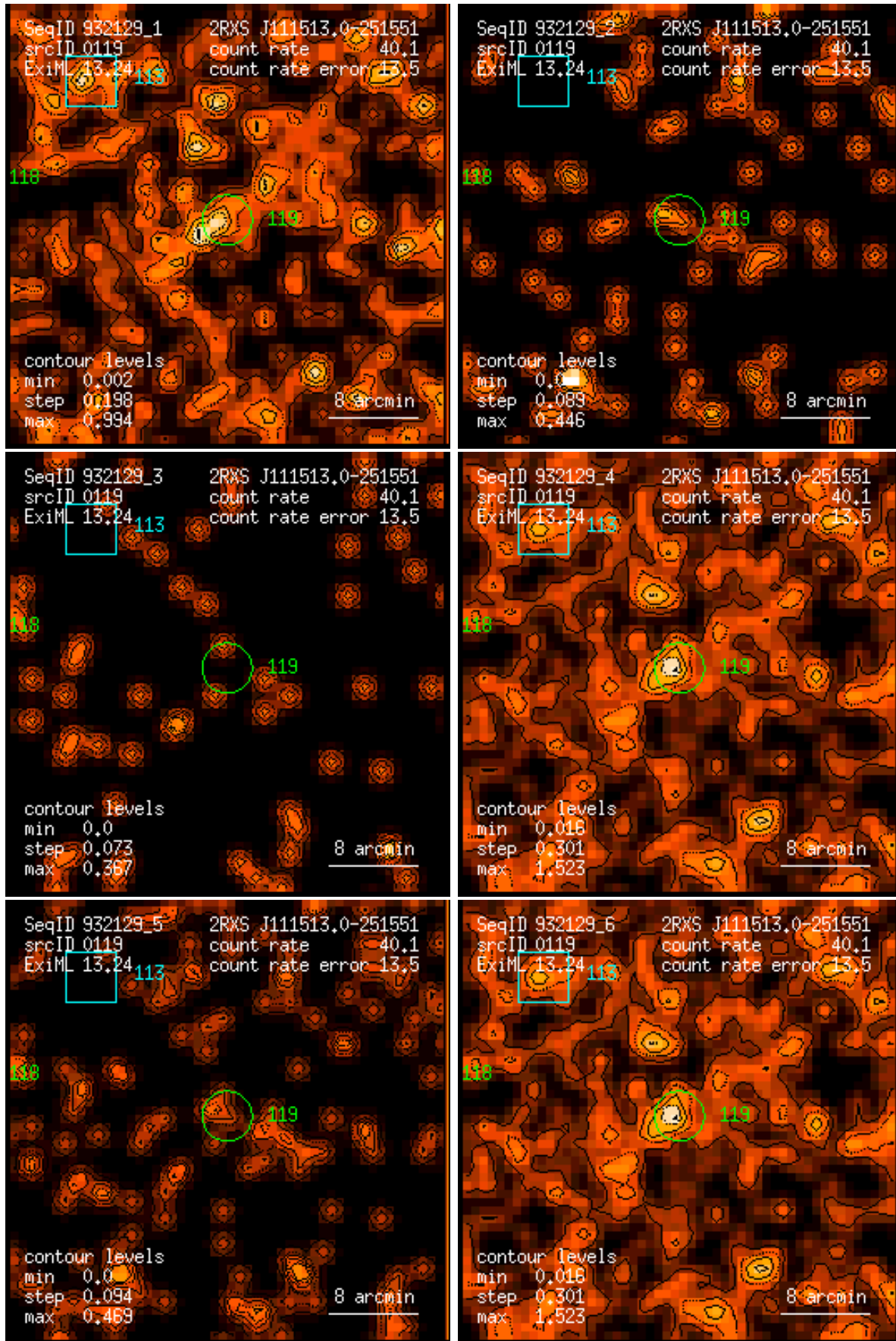
Figure 119: RASS 932129: detection 0119: band rate images, Gaussian filter: (1) PSPP channels 11 – 41, (2) 52 – 90, (3) 91 – 201, (4) 11 – 235, (5) 52 – 201, (6) 11 – 201. Broad band rates in counts/ks. Band rate contour levels in counts/ks/arcmin 2 .
