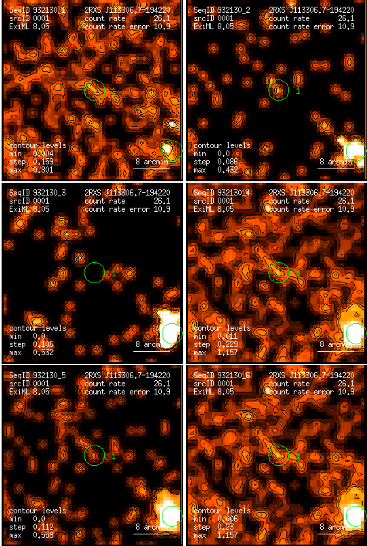
Figure 1: RASS 932130: detection 0001: band rate images, Gaussian filter: (1) PSPC channels 11 – 41, (2) 52 – 90, (3) 91 – 201, (4) 11 – 235, (5) 52 – 201, (6) 11 – 201. Broad band rates in counts/ks. Band rate contour levels in counts/ks/arcmin 2 .
