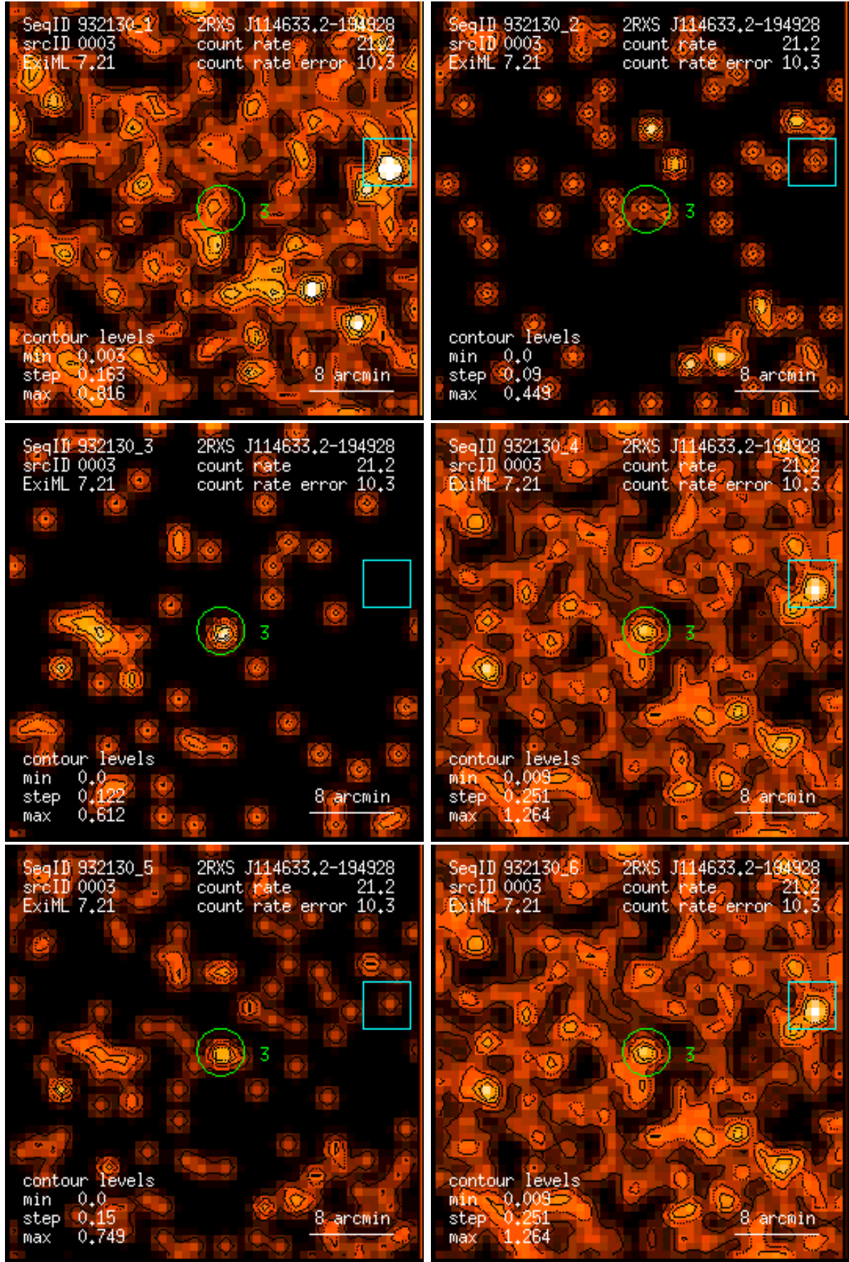
Figure 3: RASS 932130: detection 0003: band rate images, Gaussian filter: (1) PSPC channels 11 – 41, (2) 52 – 90, (3) 91 – 201, (4) 11 – 235, (5) 52 – 201, (6) 11 – 201. Broad band rates in counts/ks. Band rate contour levels in counts/ks/arcmin 2 .
