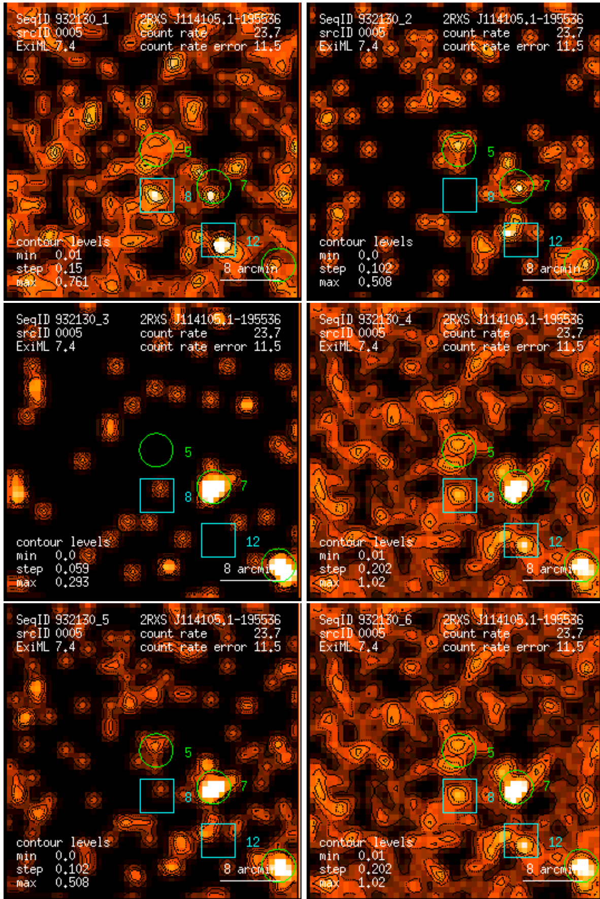
Figure 5: RASS 932130: detection 0005: band rate images, Gaussian filter: (1) PSPC channels 11 – 41, (2) 52 – 90, (3) 91 – 201, (4) 11 – 235, (5) 52 – 201, (6) 11 – 201. Broad band rates in counts/ks. Band rate contour levels in counts/ks/arcmin 2 .
