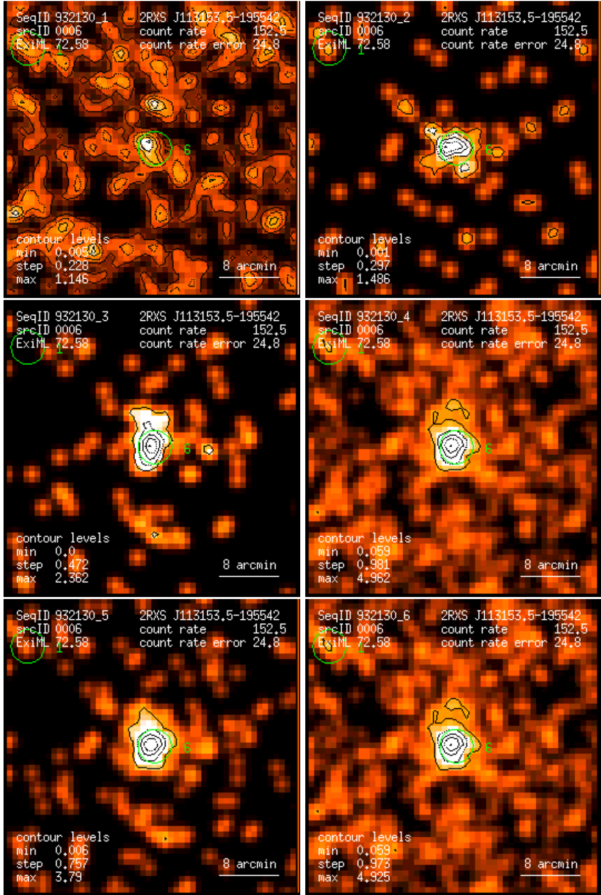
Figure 6: RASS 932130: detection 0006: band rate images, Gaussian filter: (1) PSPC channels 11 – 41, (2) 52 – 90, (3) 91 – 201, (4) 11 – 235, (5) 52 – 201, (6) 11 – 201. Broad band rates in counts/ks. Band rate contour levels in counts/ks/arcmin 2 .
