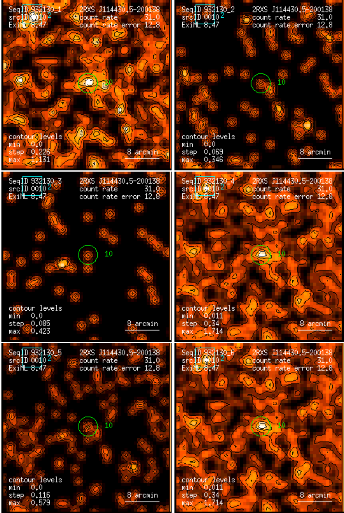
Figure 10: RASS 932130: detection 0010: band rate images, Gaussian filter: (1) PSPC channels 11 – 41, (2) 52 – 90, (3) 91 – 201, (4) 11 – 235, (5) 52 – 201, (6) 11 – 201. Broad band rates in counts/ks. Band rate contour levels in counts/ks/arcmin 2 .
