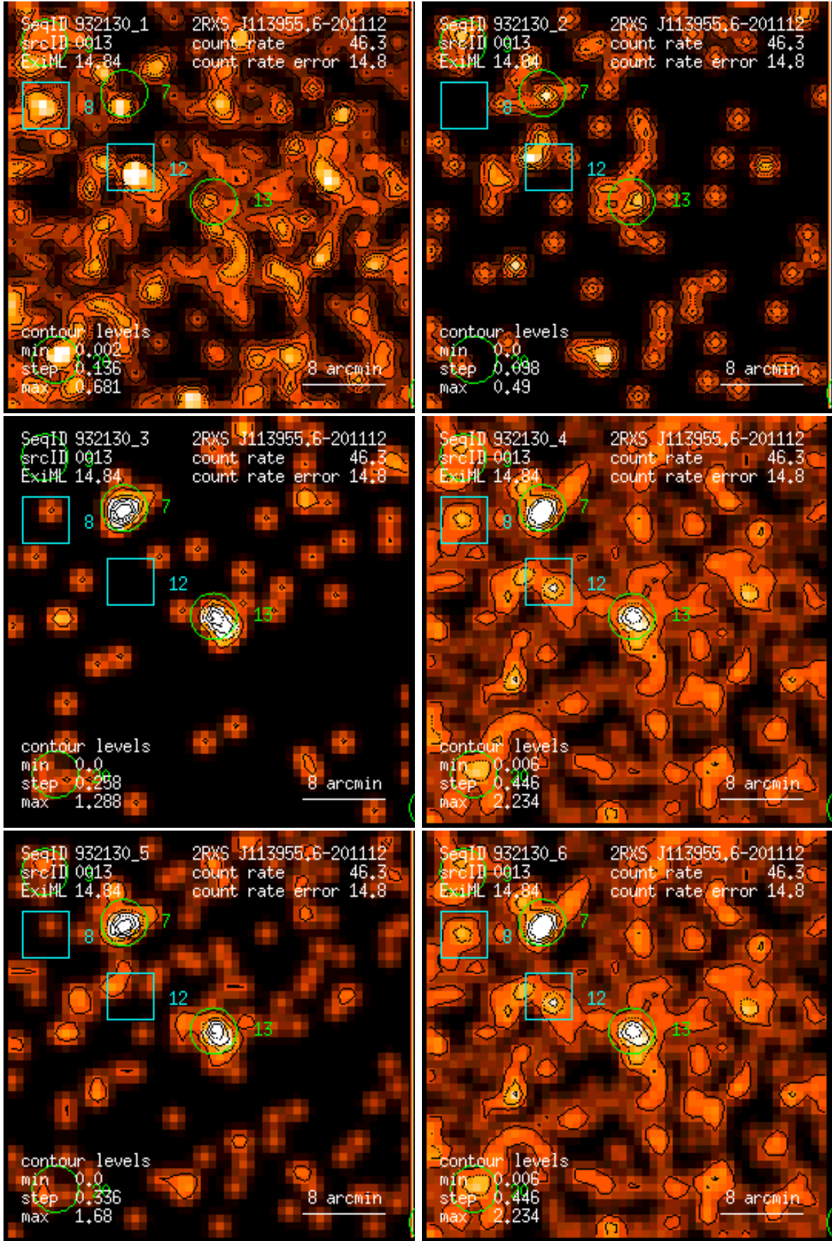
Figure 13: RASS 932130: detection 0013: band rate images, Gaussian filter: (1) PSPC channels 11 – 41, (2) 52 – 90, (3) 91 – 201, (4) 11 – 235, (5) 52 – 201, (6) 11 – 201. Broad band rates in counts/ks. Band rate contour levels in counts/ks/arcmin 2 .
