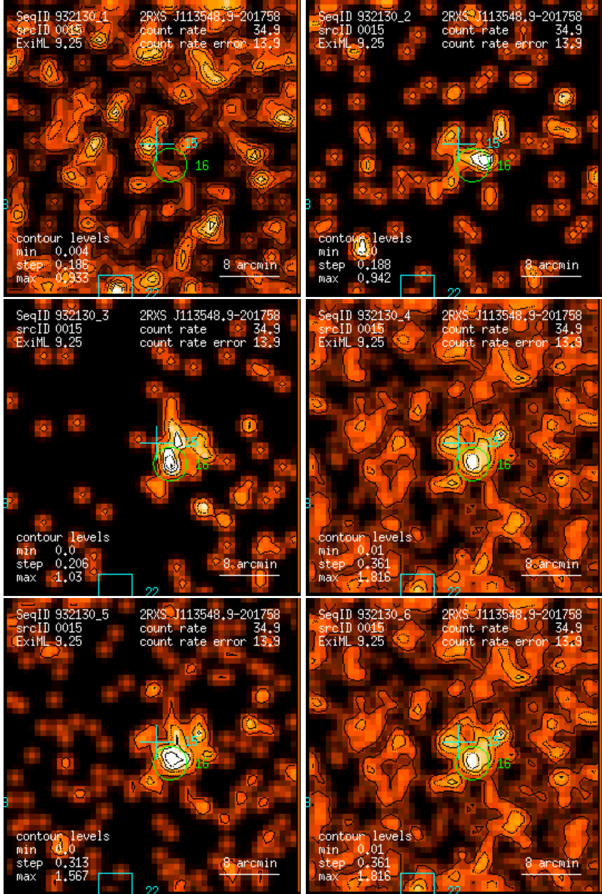
Figure 15: RASS 932130: detection 0015: band rate images, Gaussian filter: (1) PSPC channels 11 – 41, (2) 52 – 90, (3) 91 – 201, (4) 11 – 235, (5) 52 – 201, (6) 11 – 201. Broad band rates in counts/ks. Band rate contour levels in counts/ks/arcmin 2 .
