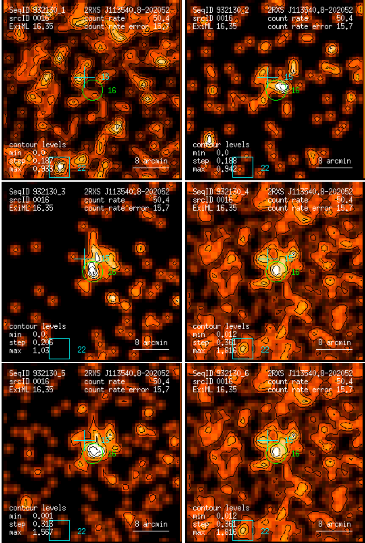
Figure 16: RASS 932130: detection 0016: band rate images, Gaussian filter: (1) PSPC channels 11 – 41, (2) 52 – 90, (3) 91 – 201, (4) 11 – 235, (5) 52 – 201, (6) 11 – 201. Broad band rates in counts/ks. Band rate contour levels in counts/ks/arcmin 2 .
