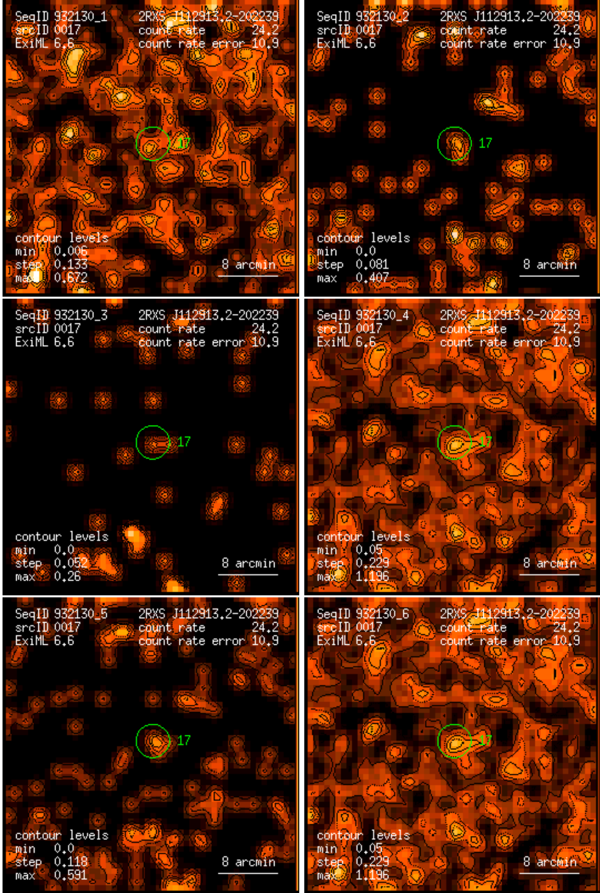
Figure 17: RASS 932130: detection 0017: band rate images, Gaussian filter: (1) PSPC channels 11 – 41, (2) 52 – 90, (3) 91 – 201, (4) 11 – 235, (5) 52 – 201, (6) 11 – 201. Broad band rates in counts/ks. Band rate contour levels in counts/ks/arcmin 2 .
