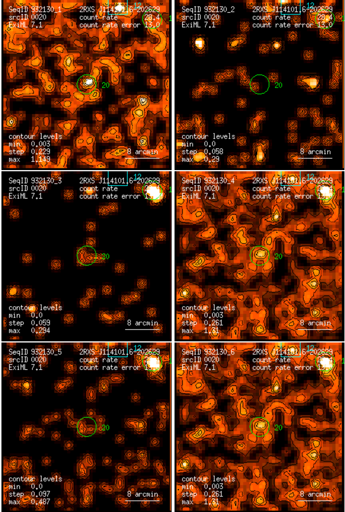
Figure 20: RASS 932130: detection 0020: band rate images, Gaussian filter: (1) PSPC channels 11 – 41, (2) 52 – 90, (3) 91 – 201, (4) 11 – 235, (5) 52 – 201, (6) 11 – 201. Broad band rates in counts/ks. Band rate contour levels in counts/ks/arcmin 2 .
