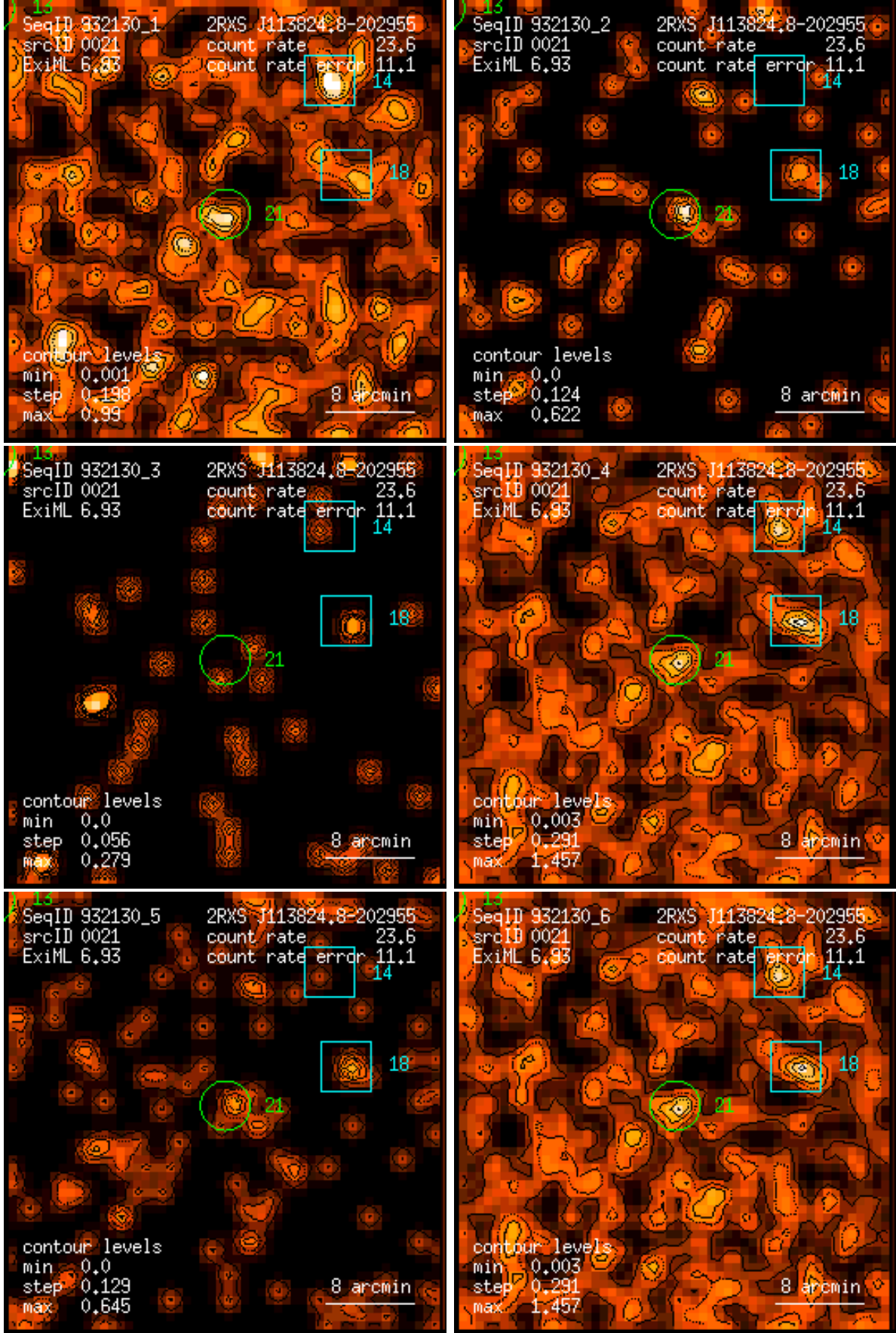
Figure 21: RASS 932130: detection 0021: band rate images, Gaussian filter: (1) PSPC channels 11 – 41, (2) 52 – 90, (3) 91 – 201, (4) 11 – 235, (5) 52 – 201, (6) 11 – 201. Broad band rates in counts/ks. Band rate contour levels in counts/ks/arcmin 2 .
