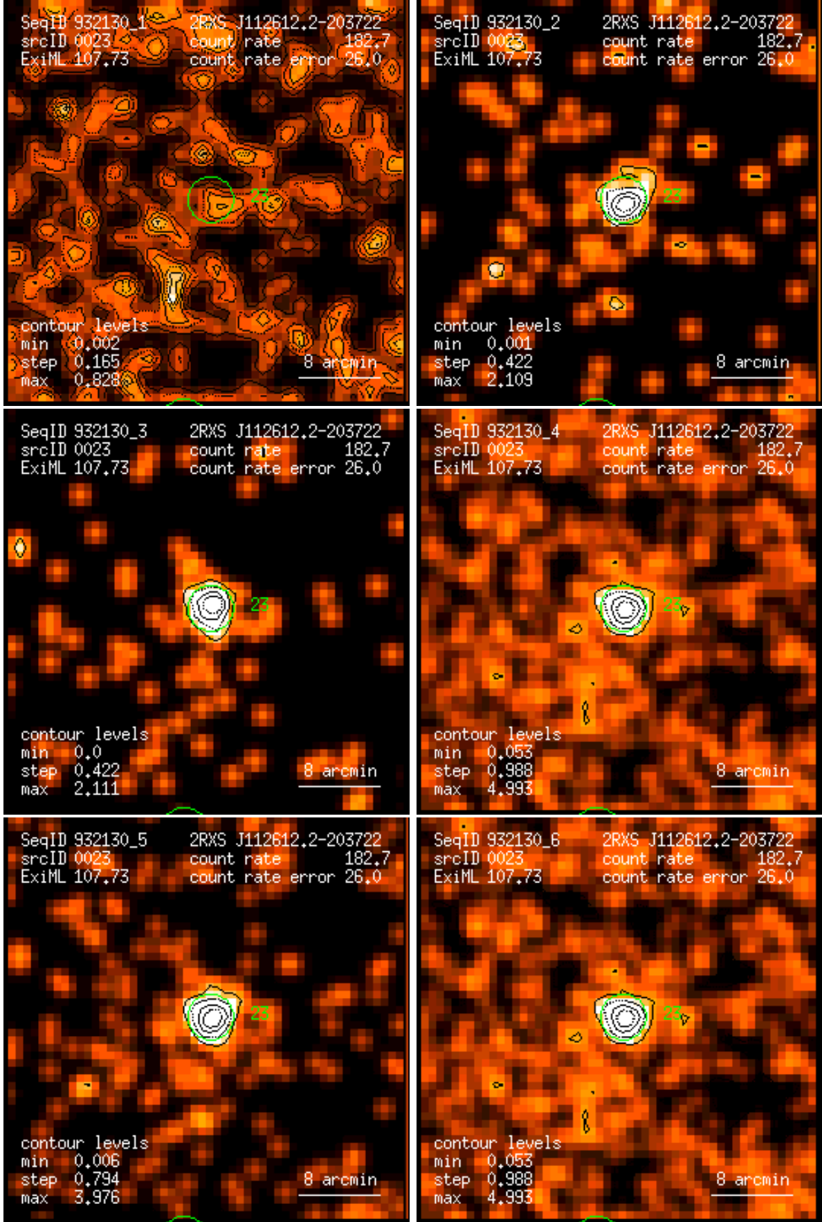
Figure 23: RASS 932130: detection 0023: band rate images, Gaussian filter: (1) PSPC channels 11 – 41, (2) 52 – 90, (3) 91 – 201, (4) 11 – 235, (5) 52 – 201, (6) 11 – 201. Broad band rates in counts/ks. Band rate contour levels in counts/ks/arcmin 2 .
