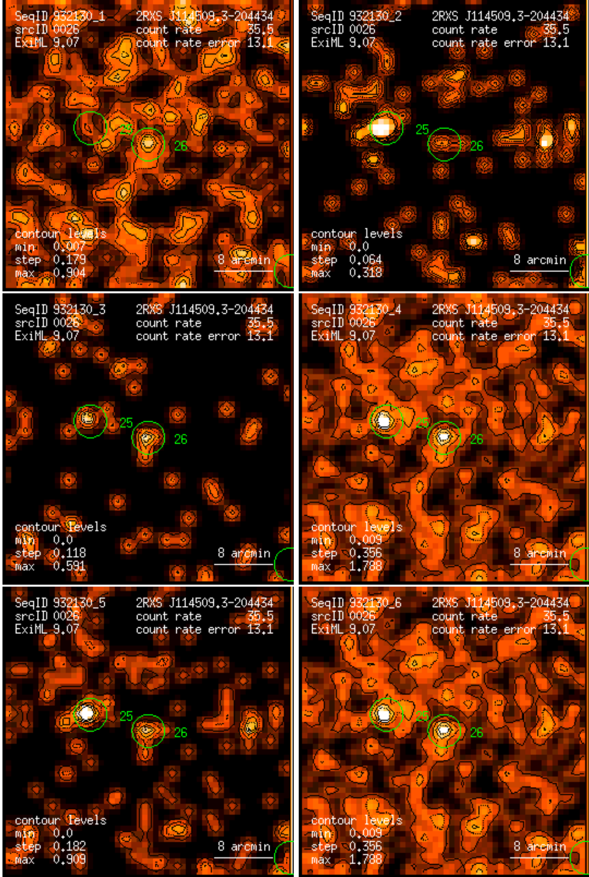
Figure 26: RASS 932130: detection 0026: band rate images, Gaussian filter: (1) PSPC channels 11 – 41, (2) 52 – 90, (3) 91 – 201, (4) 11 – 235, (5) 52 – 201, (6) 11 – 201. Broad band rates in counts/ks. Band rate contour levels in counts/ks/arcmin 2 .
