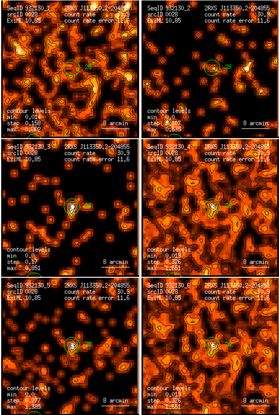
Figure 28: RASS 932130: detection 0028: band rate images, Gaussian filter: (1) PSPC channels 11 – 41, (2) 52 – 90, (3) 91 – 201, (4) 11 – 235, (5) 52 – 201, (6) 11 – 201. Broad band rates in counts/ks. Band rate contour levels in counts/ks/arcmin 2 .
