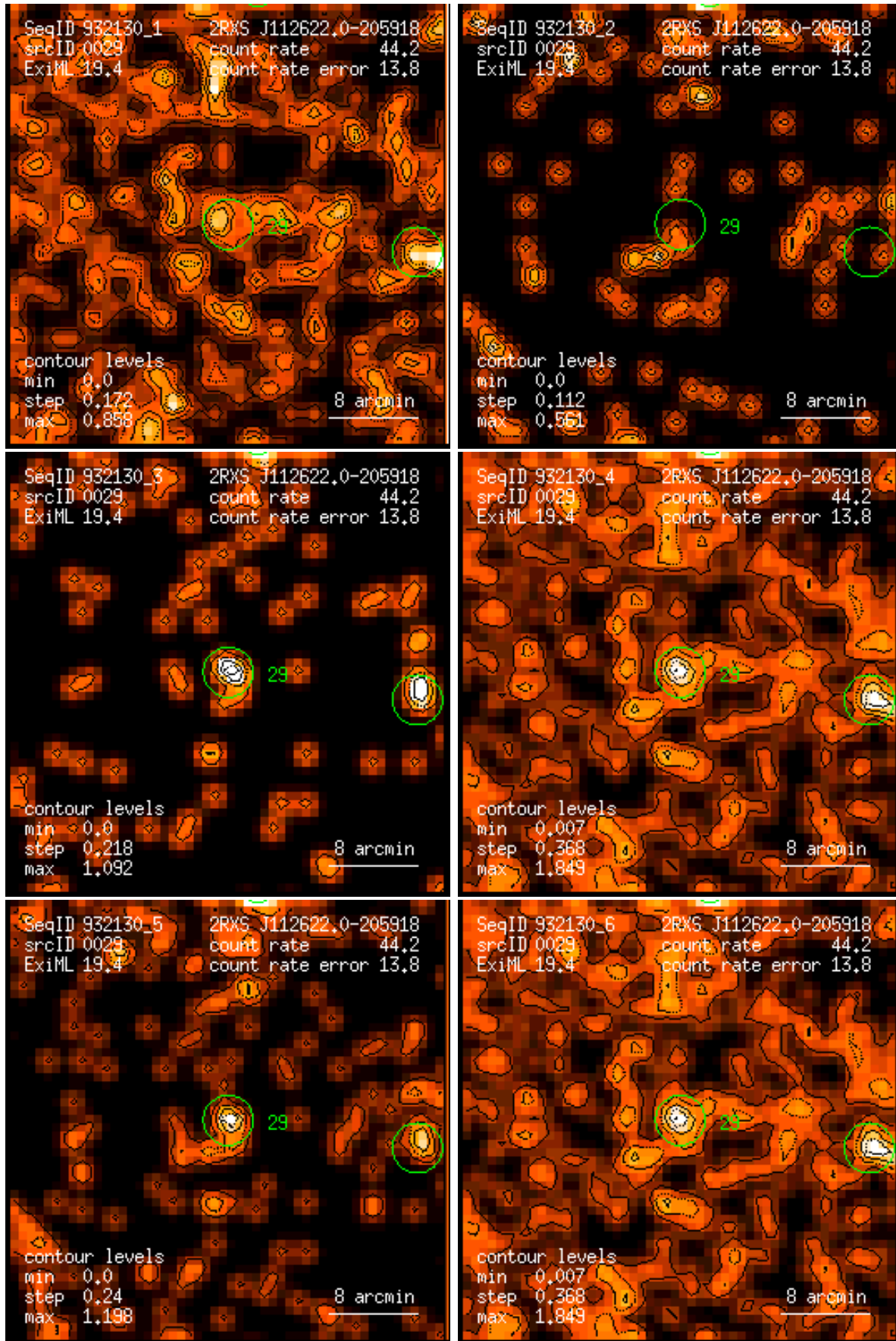
Figure 29: RASS 932130: detection 0029: band rate images, Gaussian filter: (1) PSPC channels 11 – 41, (2) 52 – 90, (3) 91 – 201, (4) 11 – 235, (5) 52 – 201, (6) 11 – 201. Broad band rates in counts/ks. Band rate contour levels in counts/ks/arcmin 2 .
