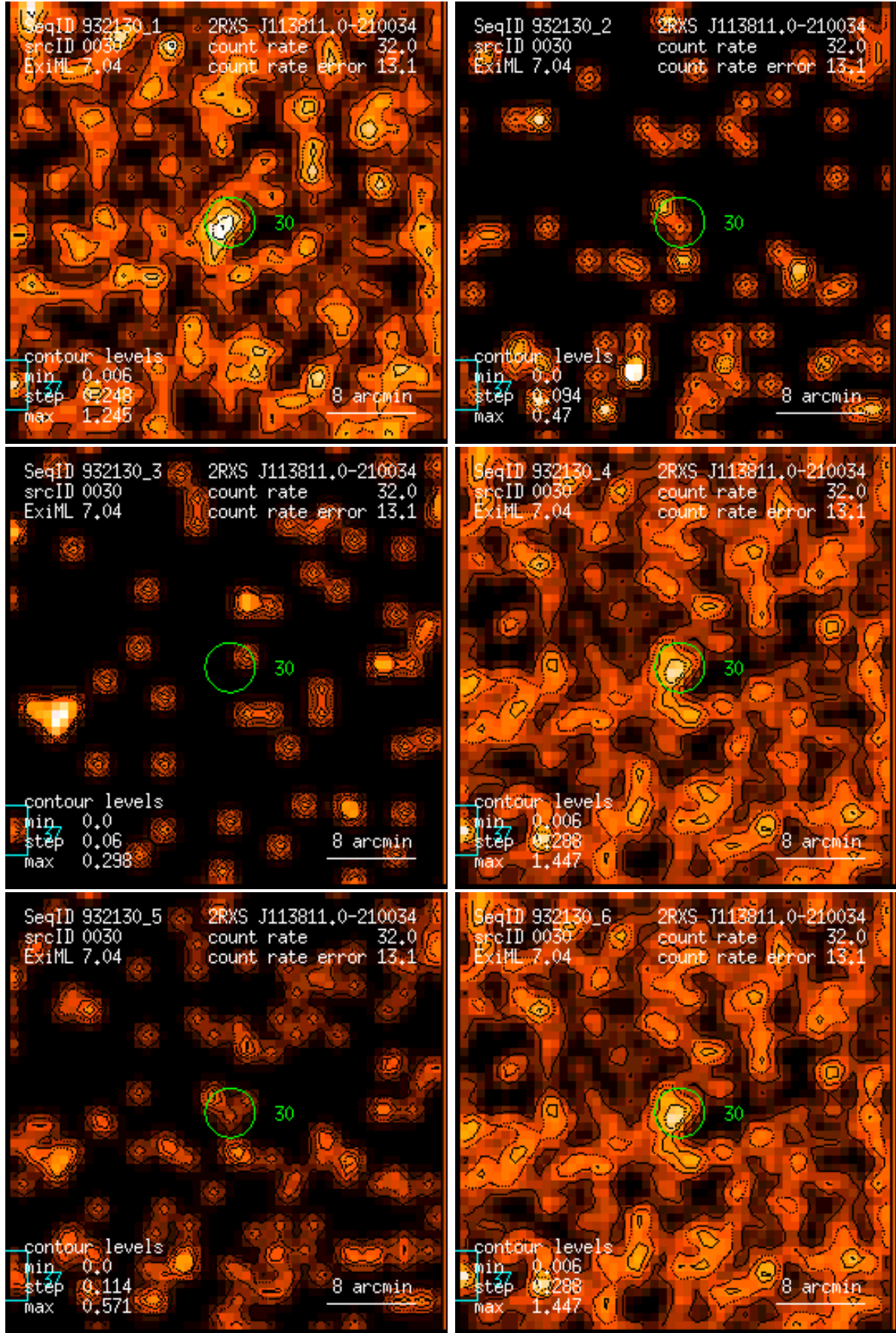
Figure 30: RASS 932130: detection 0030: band rate images, Gaussian filter: (1) PSPC channels 11 – 41, (2) 52 – 90, (3) 91 – 201, (4) 11 – 235, (5) 52 – 201, (6) 11 – 201. Broad band rates in counts/ks. Band rate contour levels in counts/ks/arcmin 2 .
