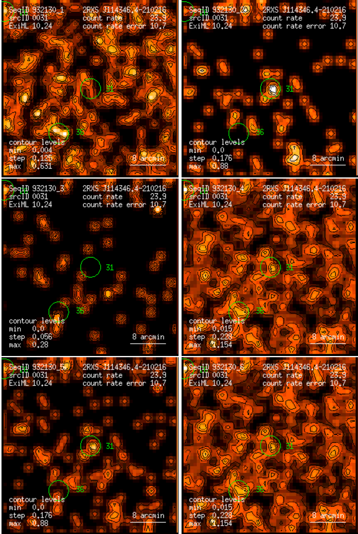
Figure 31: RASS 932130: detection 0031: band rate images, Gaussian filter: (1) PSPC channels 11 – 41, (2) 52 – 90, (3) 91 – 201, (4) 11 – 235, (5) 52 – 201, (6) 11 – 201. Broad band rates in counts/ks. Band rate contour levels in counts/ks/arcmin 2 .
