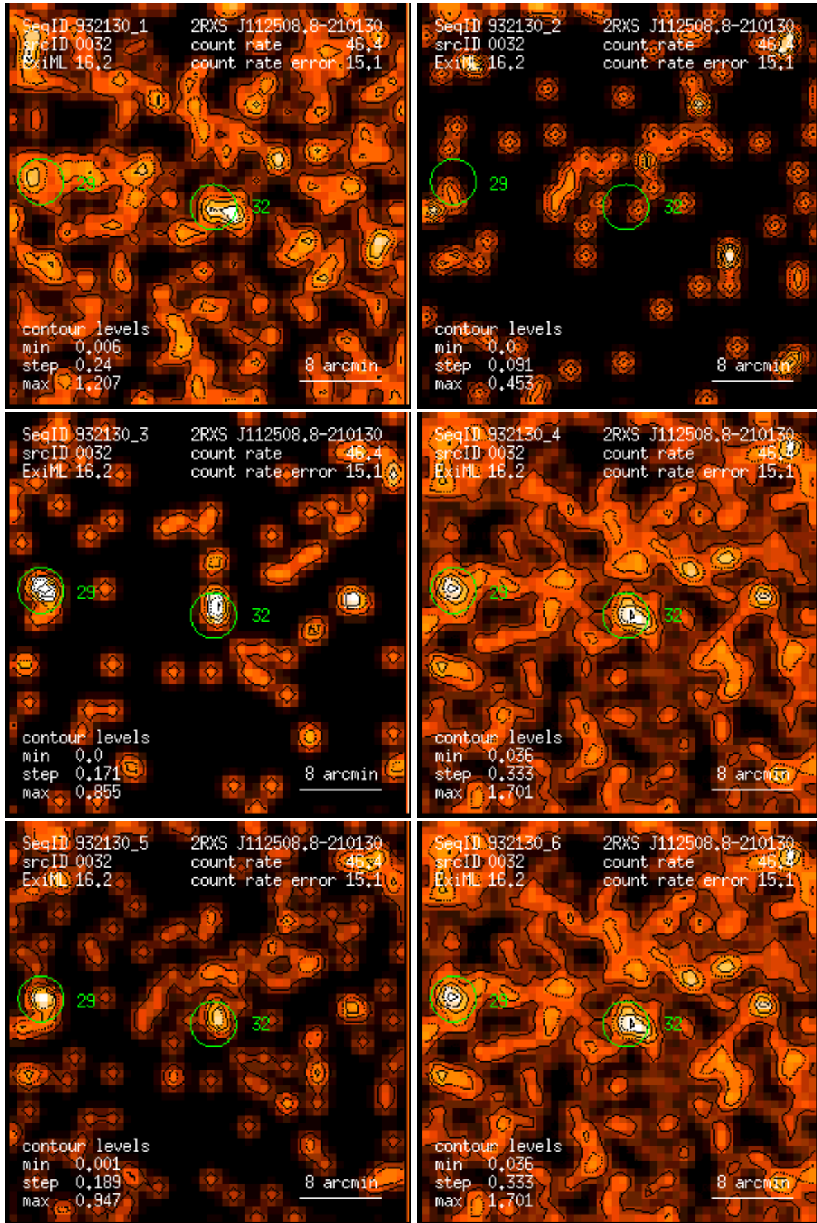
Figure 32: RASS 932130: detection 0032: band rate images, Gaussian filter: (1) PSPC channels 11 – 41, (2) 52 – 90, (3) 91 – 201, (4) 11 – 235, (5) 52 – 201, (6) 11 – 201. Broad band rates in counts/ks. Band rate contour levels in counts/ks/arcmin 2 .
