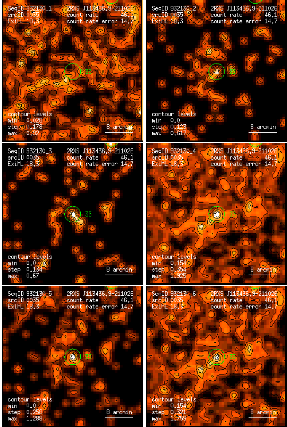
Figure 35: RASS 932130: detection 0035: band rate images, Gaussian filter: (1) PSPC channels 11 – 41, (2) 52 – 90, (3) 91 – 201, (4) 11 – 235, (5) 52 – 201, (6) 11 – 201. Broad band rates in counts/ks. Band rate contour levels in counts/ks/arcmin 2 .
