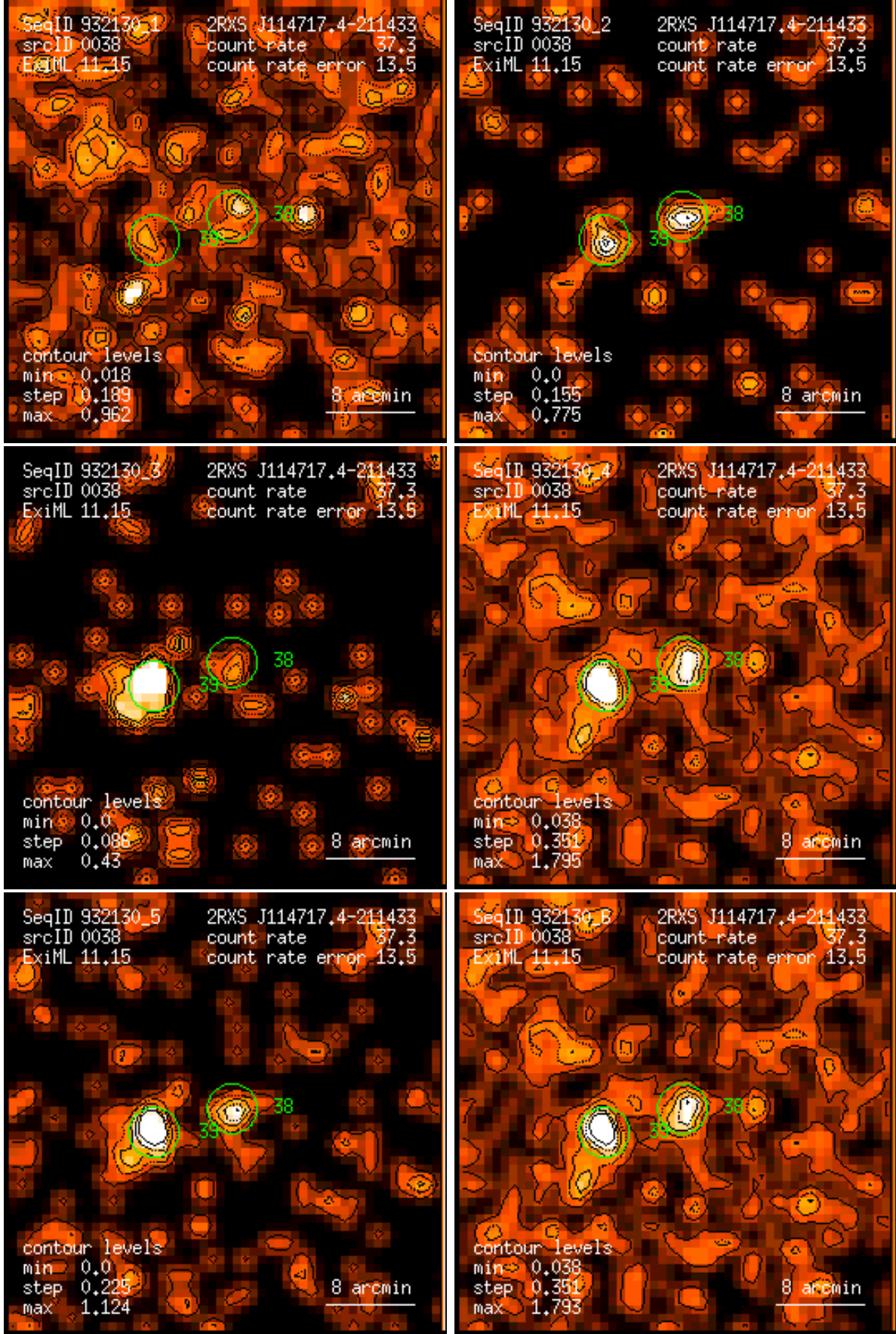
Figure 38: RASS 932130: detection 0038: band rate images, Gaussian filter: (1) PSPC channels 11 – 41, (2) 52 – 90, (3) 91 – 201, (4) 11 – 235, (5) 52 – 201, (6) 11 – 201. Broad band rates in counts/ks. Band rate contour levels in counts/ks/arcmin 2 .
