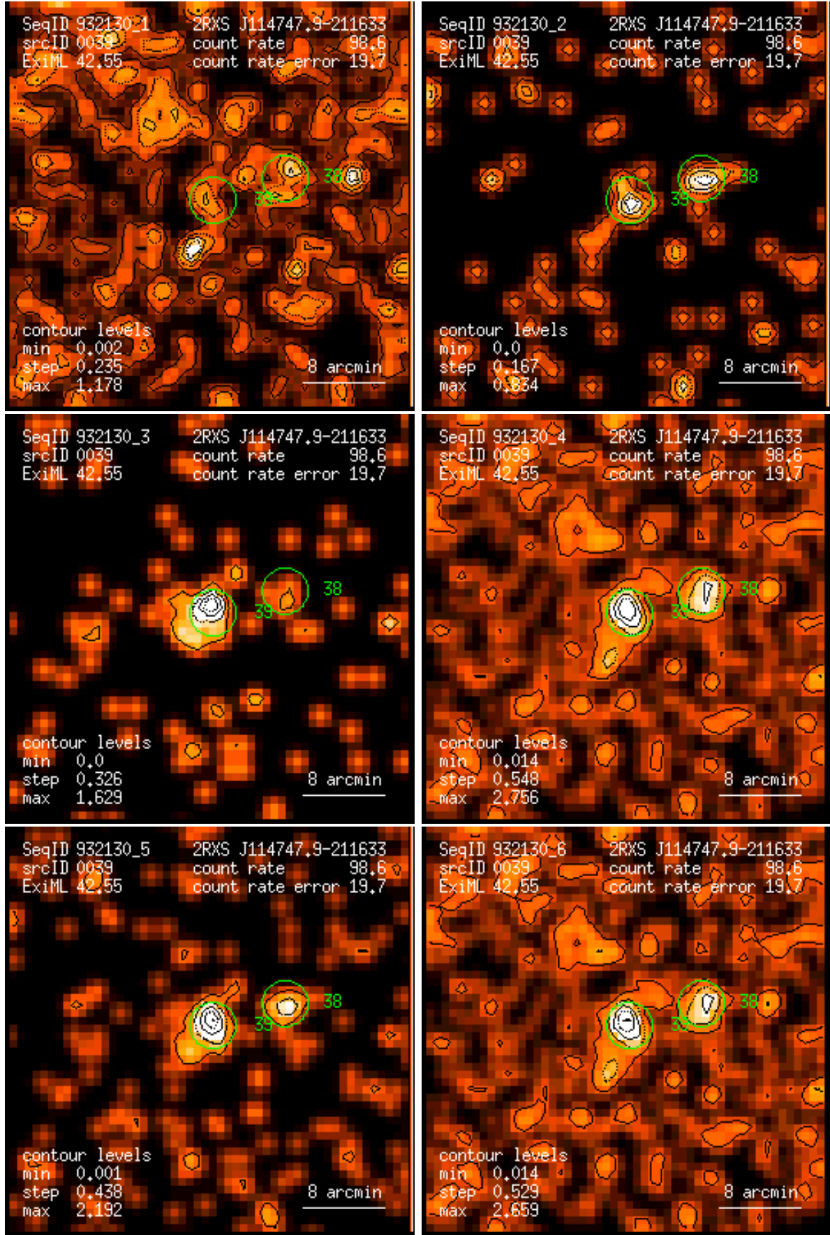
Figure 39: RASS 932130: detection 0039: band rate images, Gaussian filter: (1) PSPC channels 11 – 41, (2) 52 – 90, (3) 91 – 201, (4) 11 – 235, (5) 52 – 201, (6) 11 – 201. Broad band rates in counts/ks. Band rate contour levels in counts/ks/arcmin 2 .
