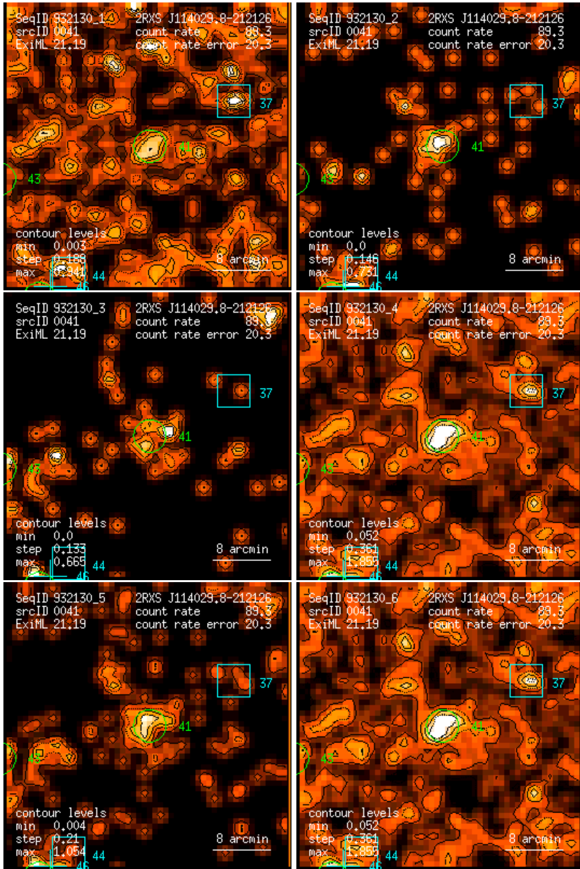
Figure 41: RASS 932130: detection 0041: band rate images, Gaussian filter: (1) PSPC channels 11 – 41, (2) 52 – 90, (3) 91 – 201, (4) 11 – 235, (5) 52 – 201, (6) 11 – 201. Broad band rates in counts/ks. Band rate contour levels in counts/ks/arcmin 2 .
